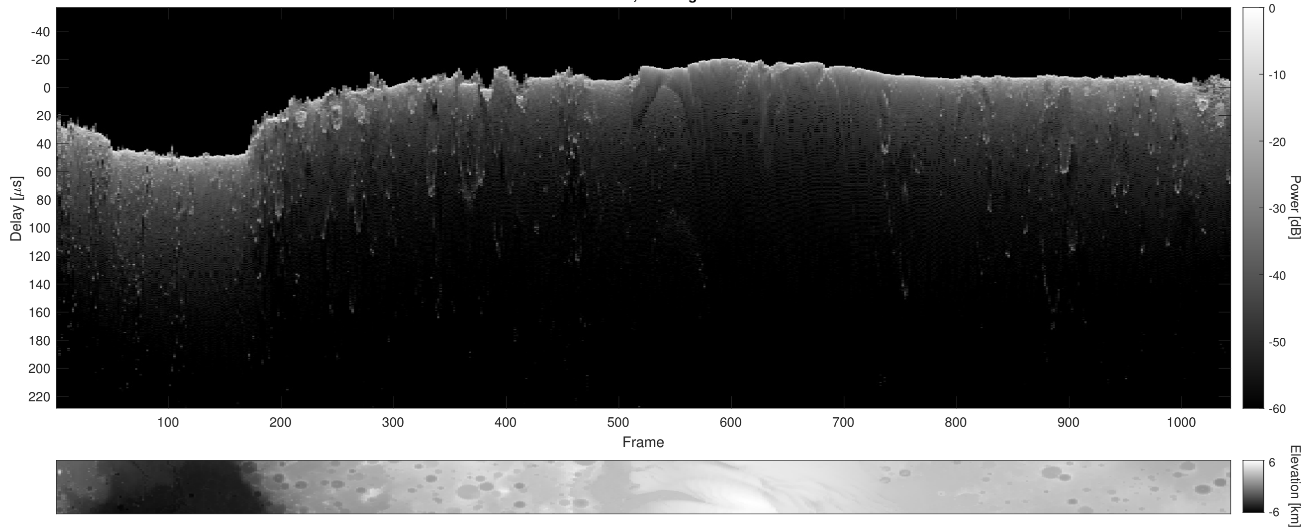
Orbit 8783, Cluttergram
