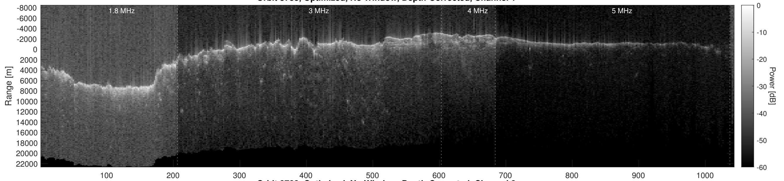
Orbit 8783, Optimized, No Window, Depth-Corrected, Channel 2
