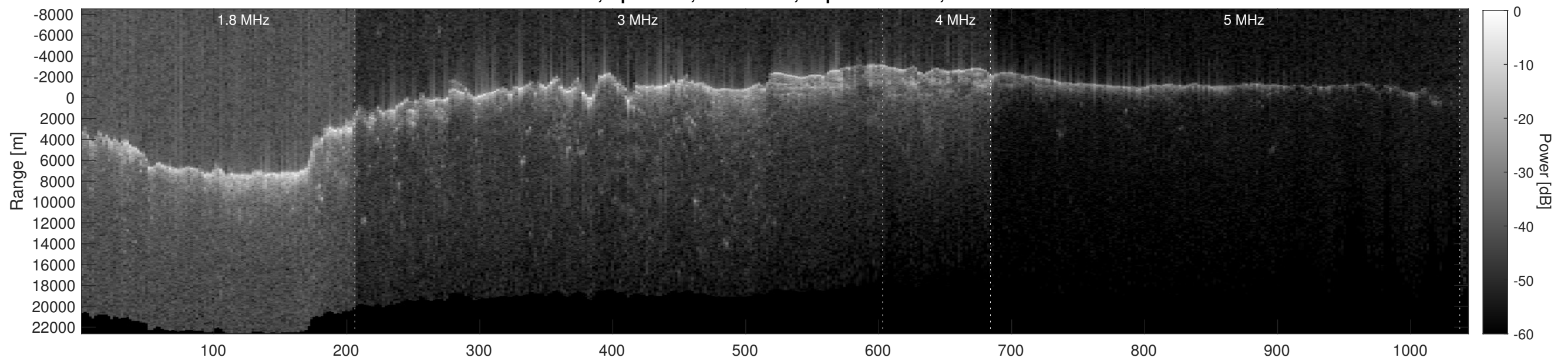
Orbit 8783, Depth-Corrected Cluttergram
