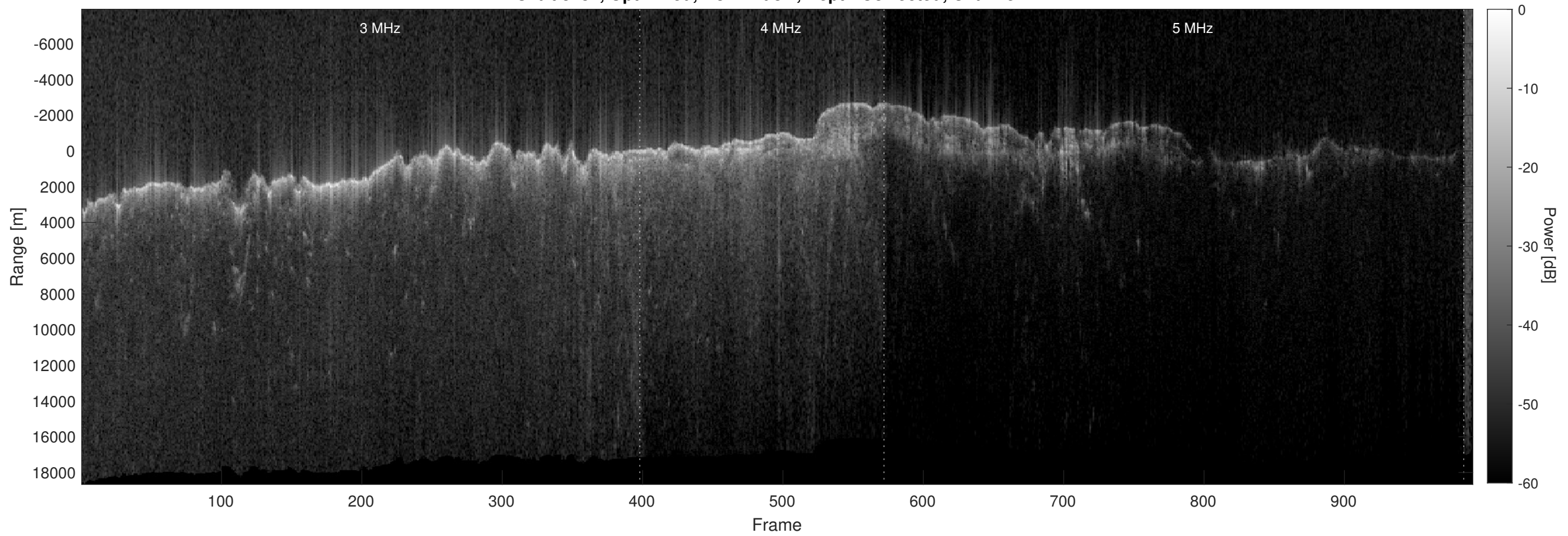
Orbit 8784, Optimized, No Window, Depth-Corrected, Channel 2
