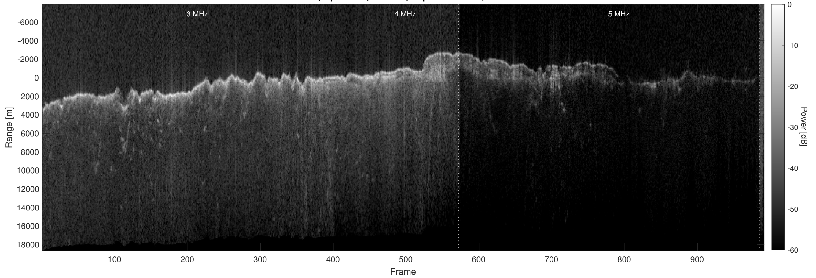
Orbit 8784, Optimized, Window, Depth-Corrected, Channel 2
