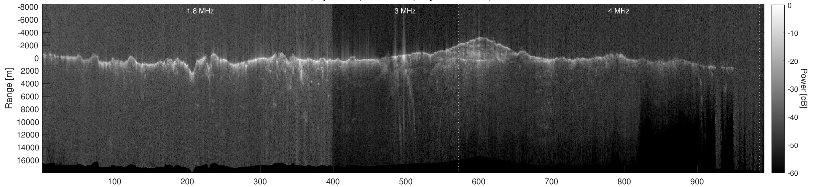
Orbit 8785, Depth-Corrected Cluttergram
