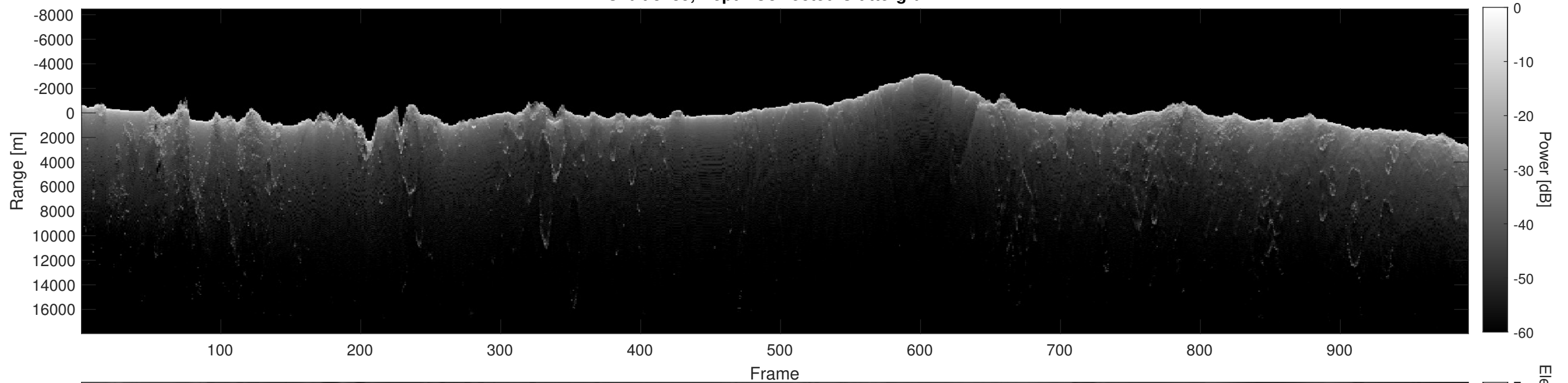
Orbit 8785, Depth-Corrected Cluttergram
