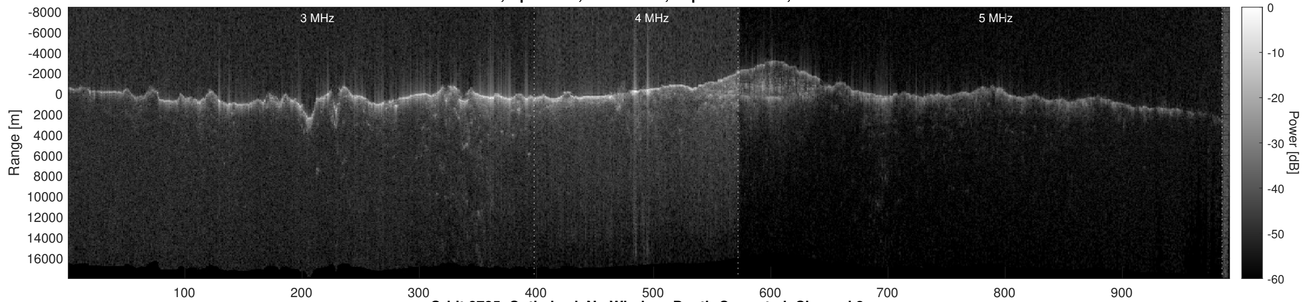
Orbit 8785, Optimized, No Window, Depth-Corrected, Channel 2
