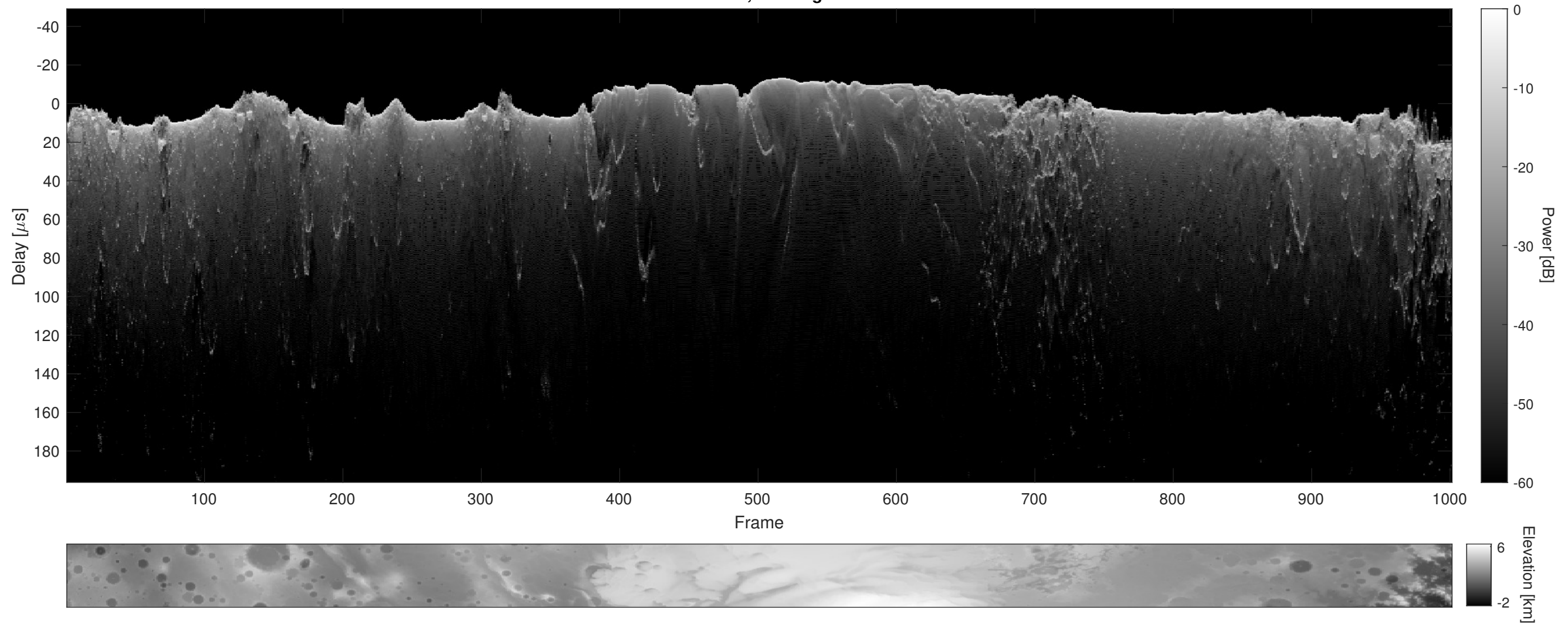
Orbit 8786, Cluttergram
