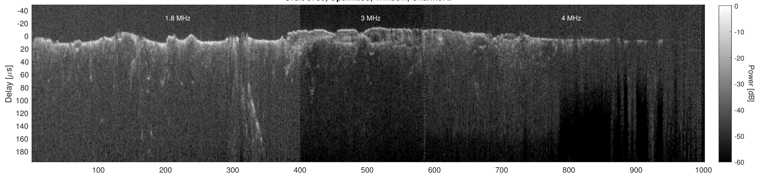
Orbit 8786, Cluttergram
