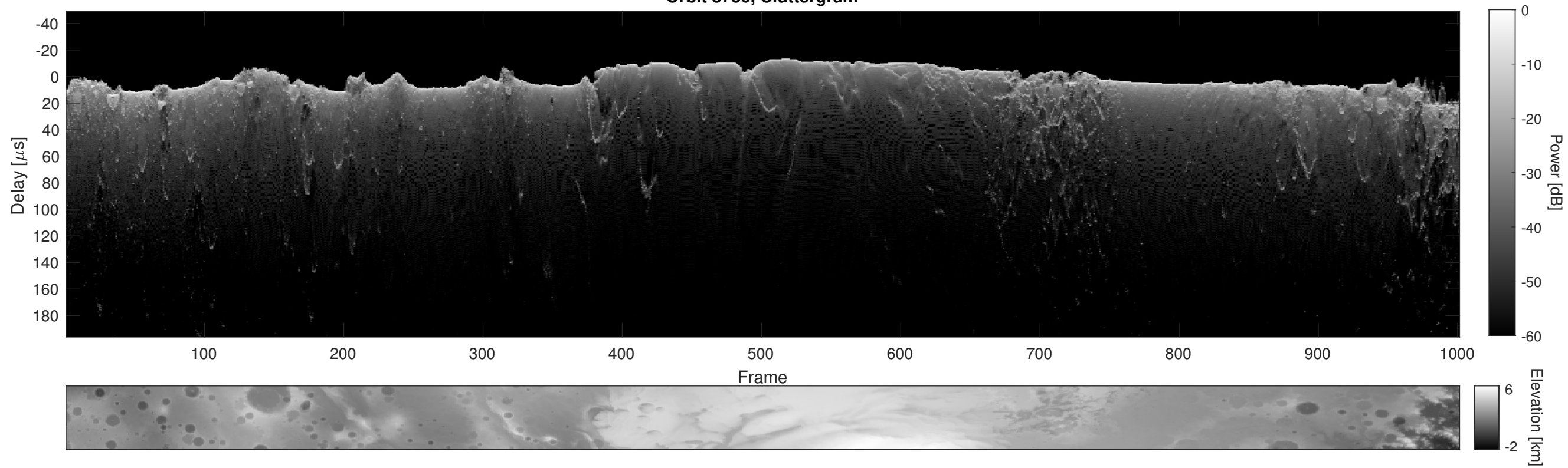
Orbit 8786, Cluttergram
