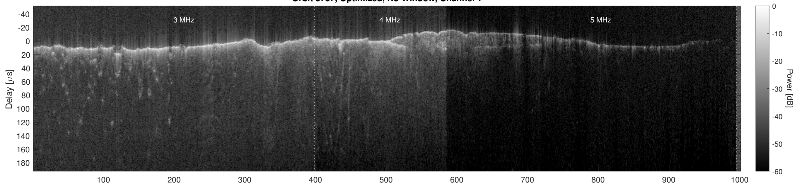
Orbit 8787, Optimized, No Window, Channel 2
