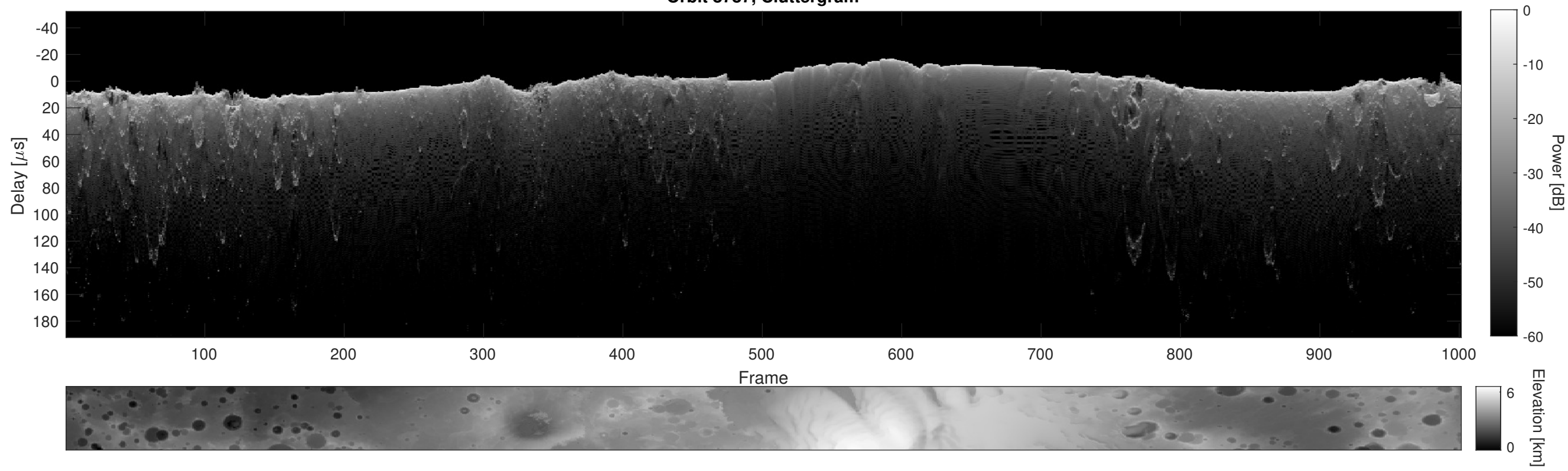
Orbit 8787, Cluttergram
