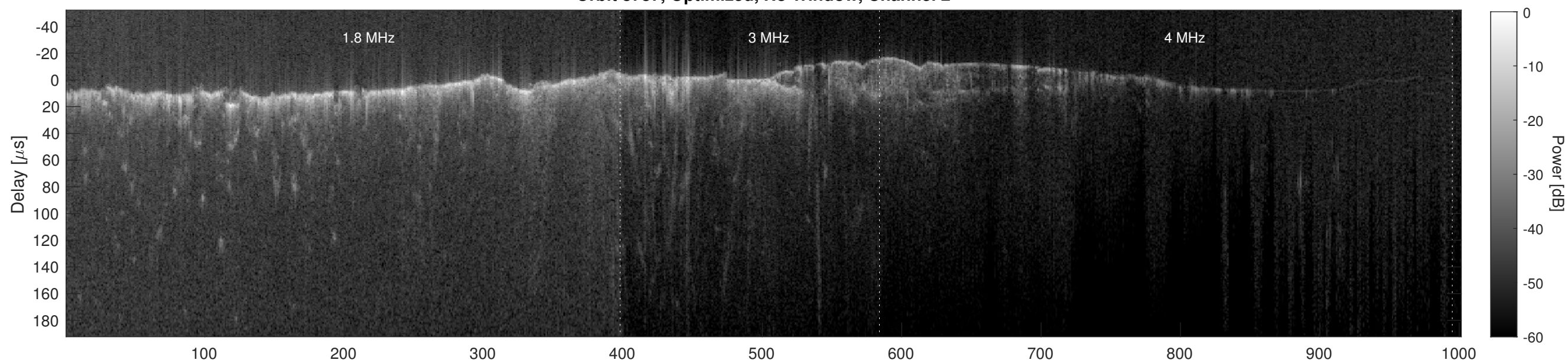
Orbit 8787, Cluttergram
