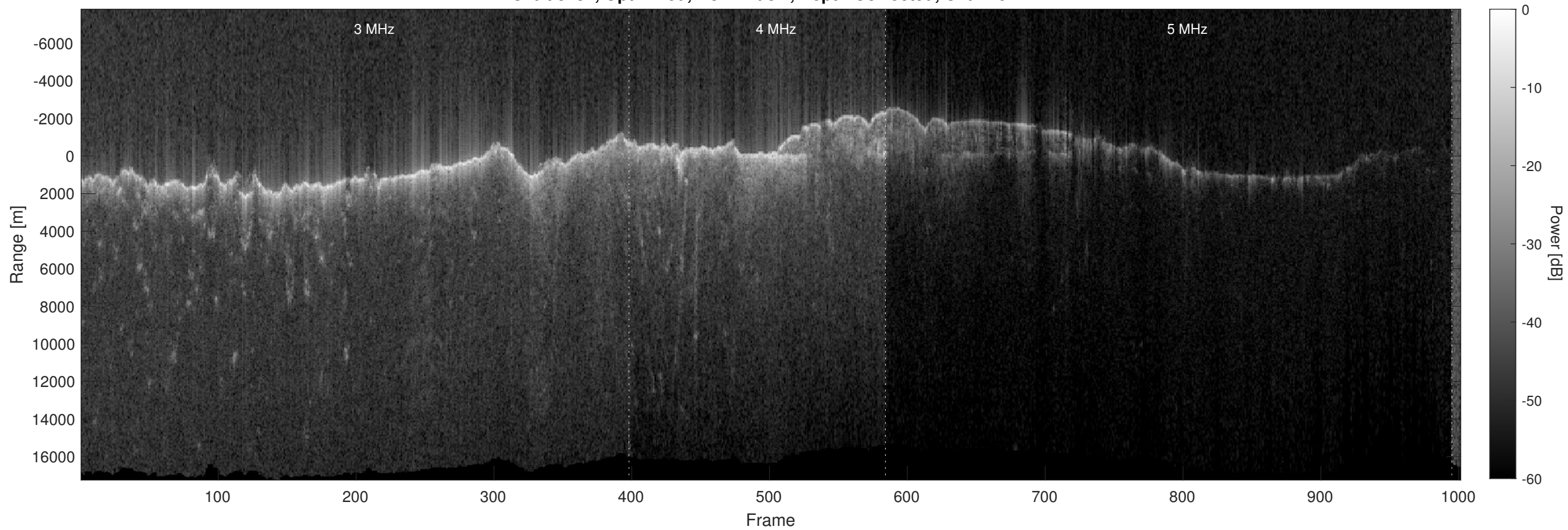
Orbit 8787, Optimized, No Window, Depth-Corrected, Channel 2
