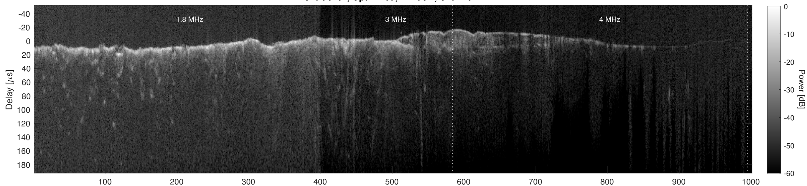
Orbit 8787, Cluttergram
