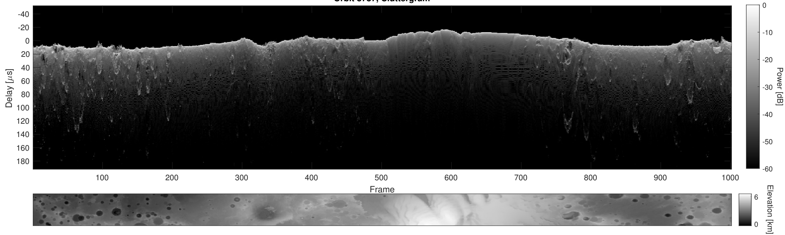
Orbit 8787, Cluttergram
