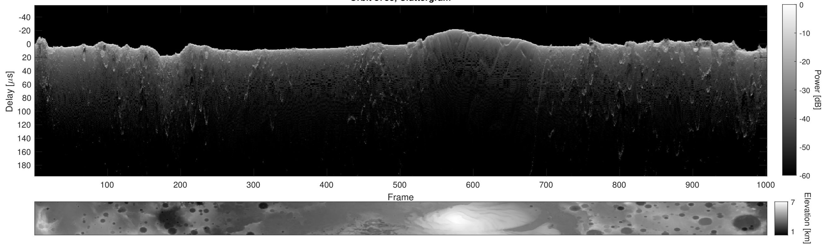
Orbit 8788, Cluttergram
