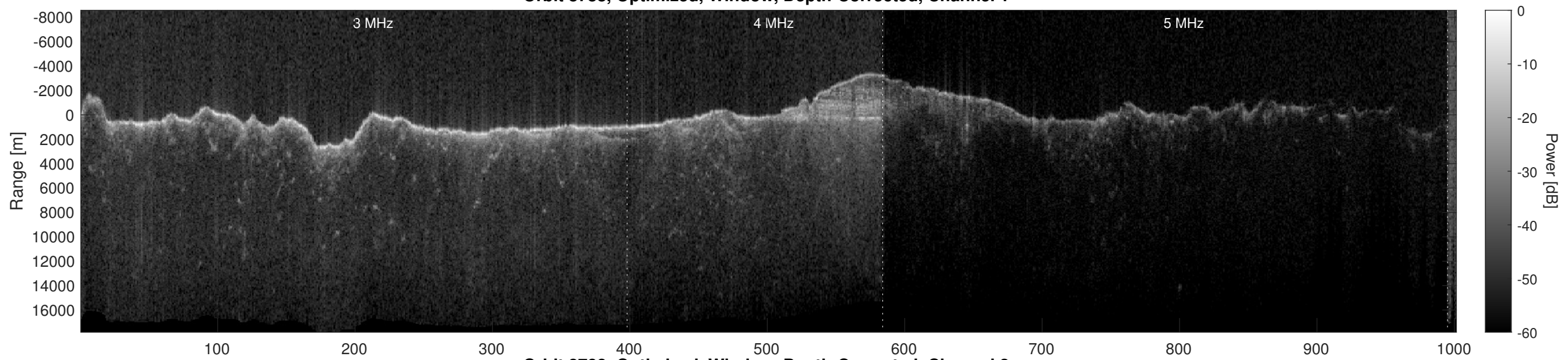
Orbit 8788, Optimized, Window, Depth-Corrected, Channel 2
