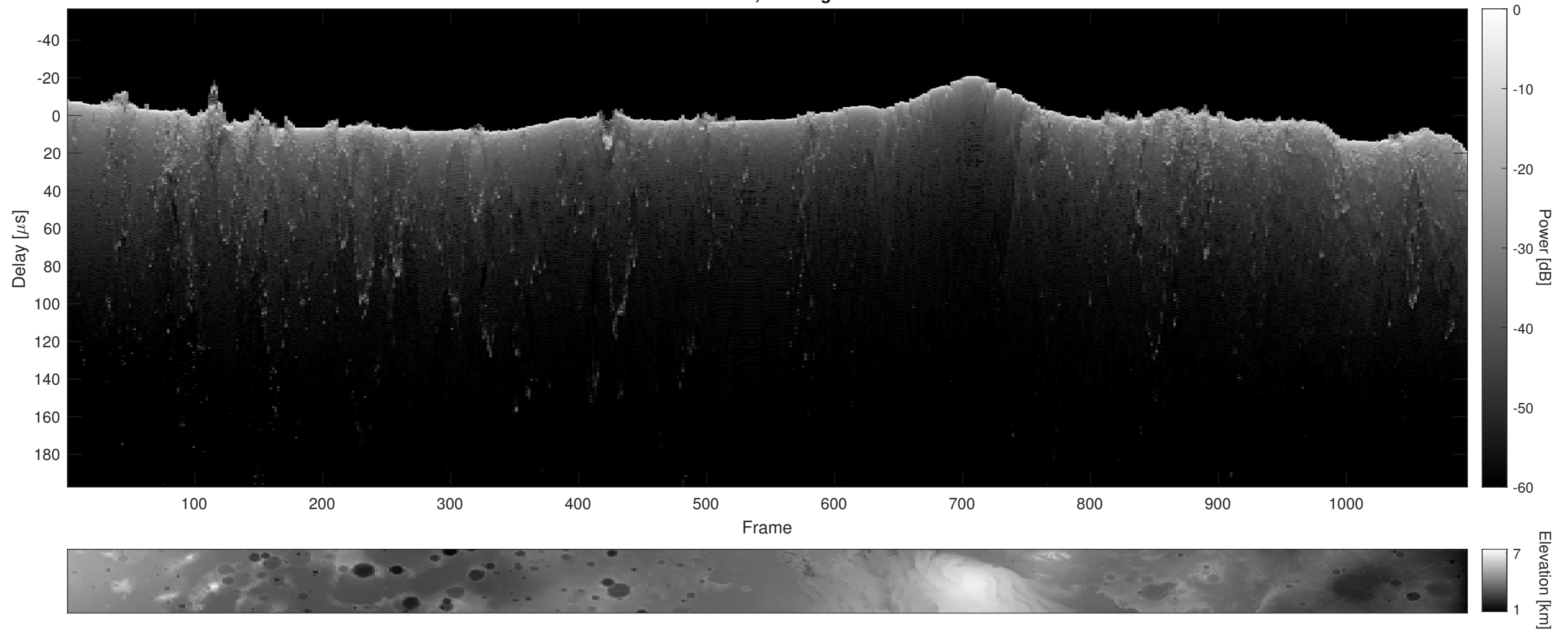
Orbit 8792, Cluttergram
