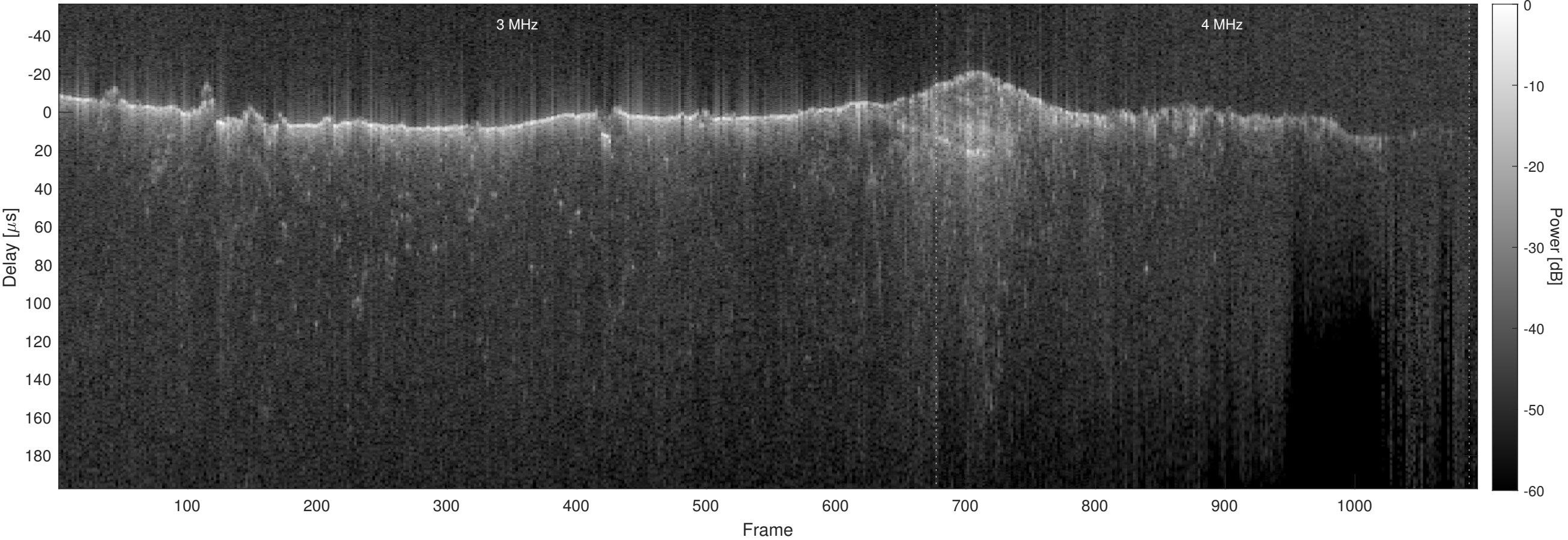
Orbit 8792, Optimized, No Window, Channel 2
