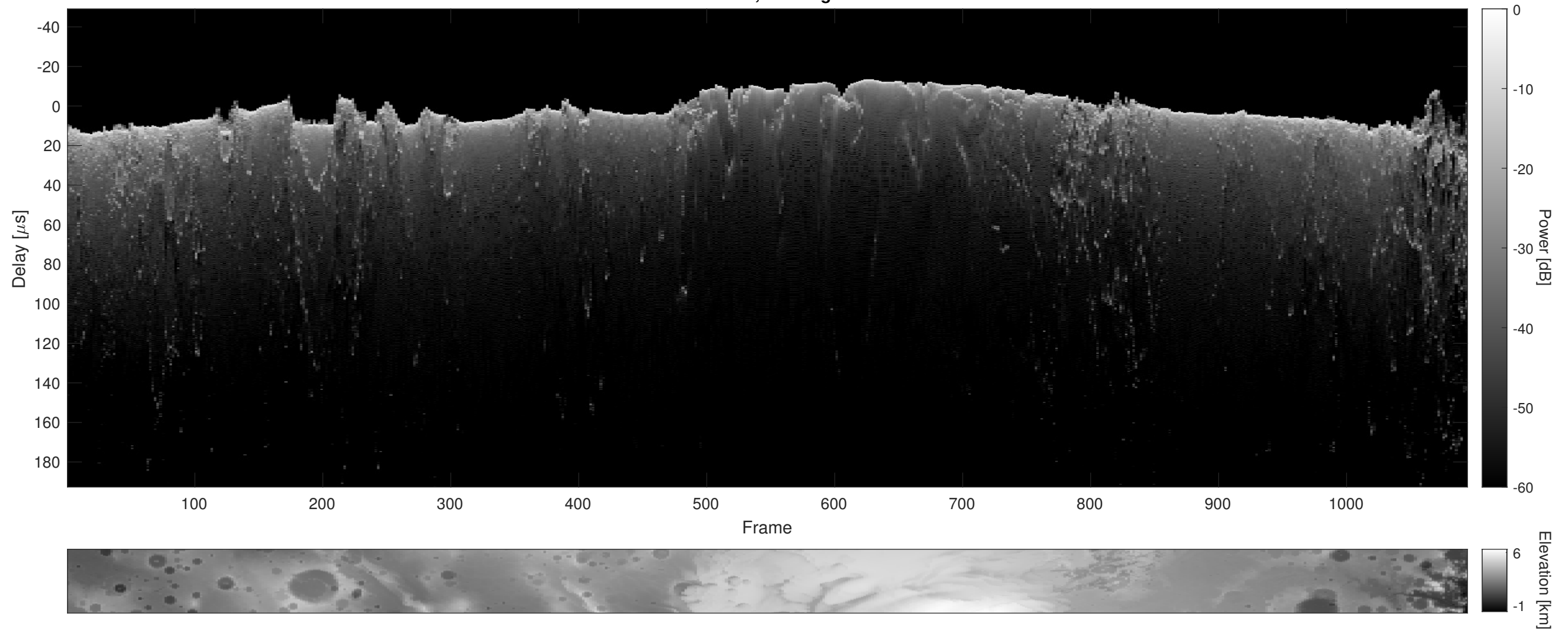
Orbit 8793, Cluttergram
