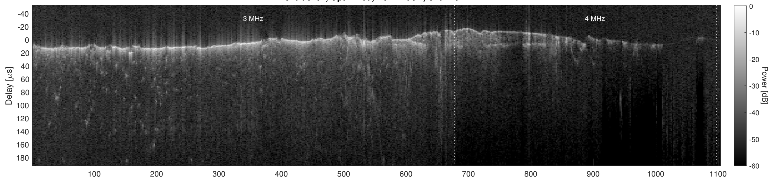
Orbit 8794, Cluttergram
