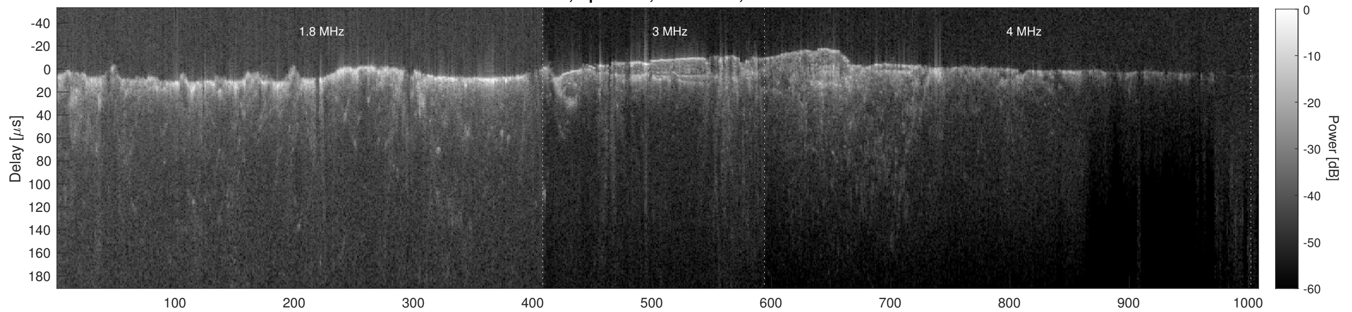
Orbit 8796, Cluttergram
