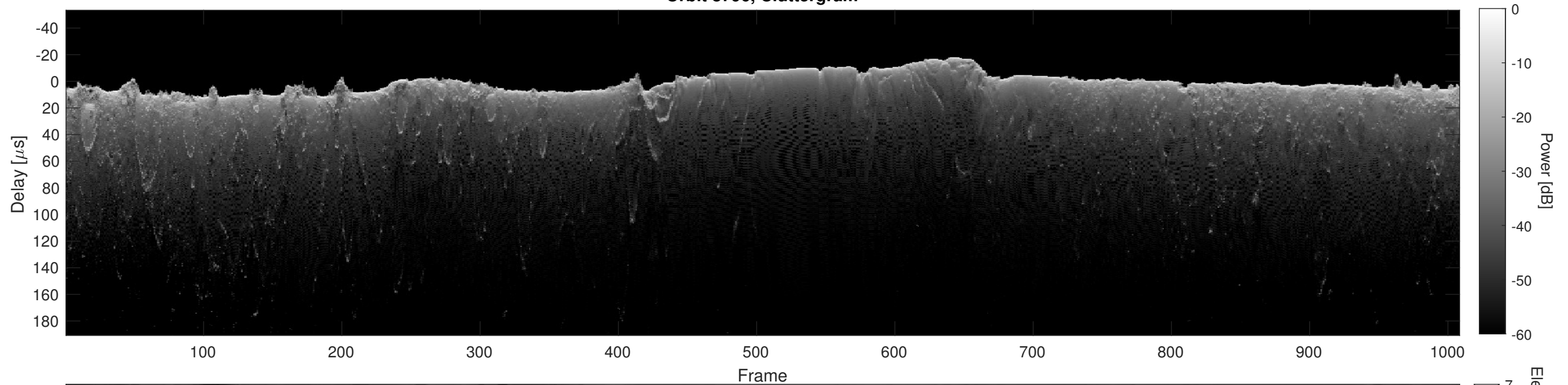
Orbit 8796, Cluttergram
