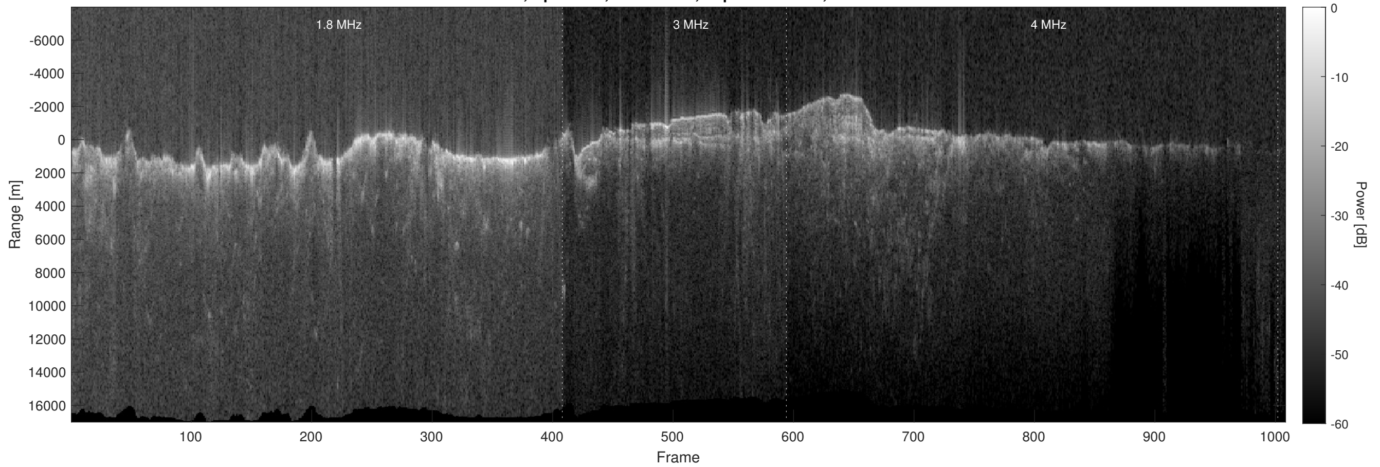
Orbit 8796, Optimized, No Window, Depth-Corrected, Channel 2
