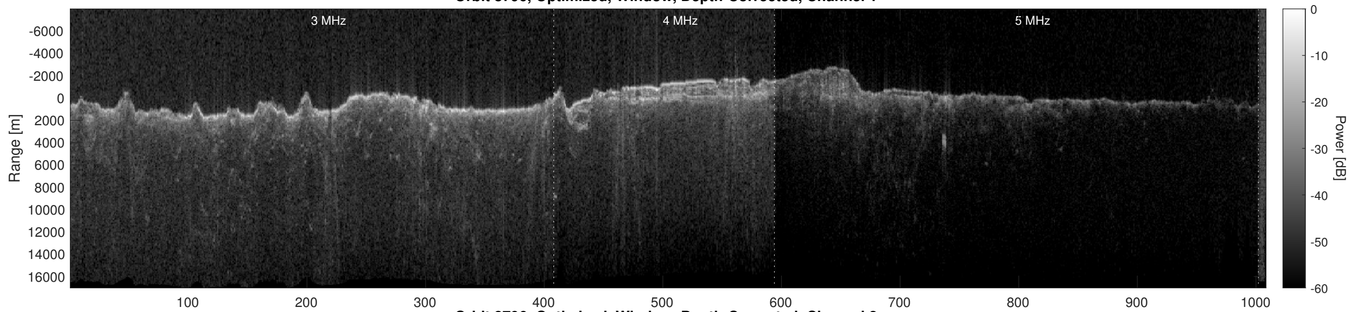
Orbit 8796, Optimized, Window, Depth-Corrected, Channel 2
