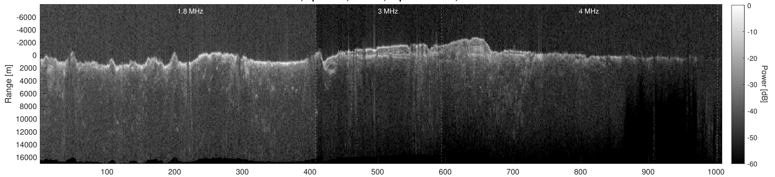
Orbit 8796, Depth-Corrected Cluttergram
