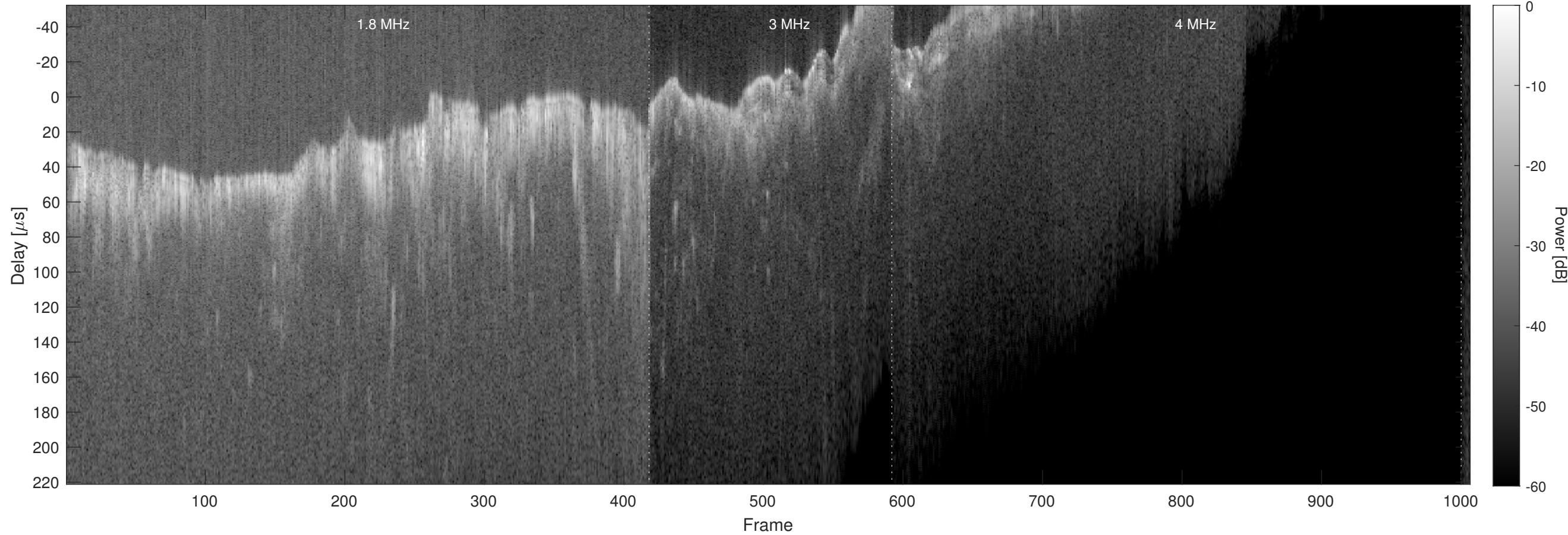
Orbit 8797, Chapman, No Window, Channel 2
