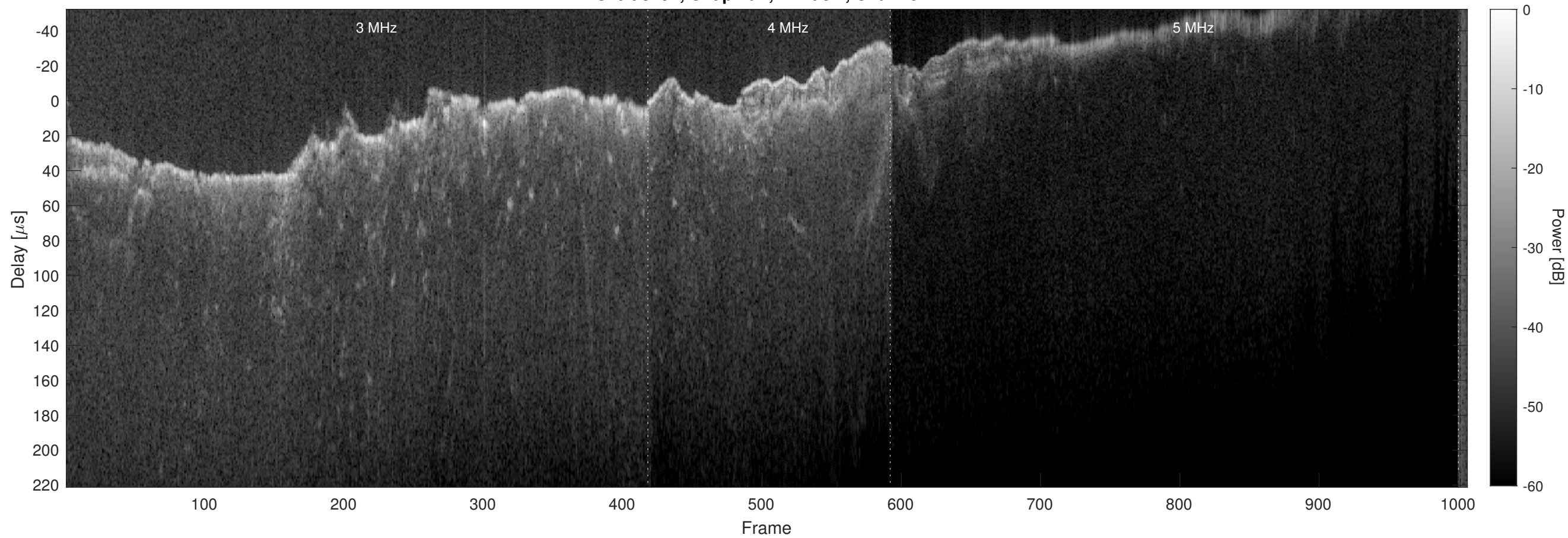
Orbit 8797, Chapman, Window, Channel 2
