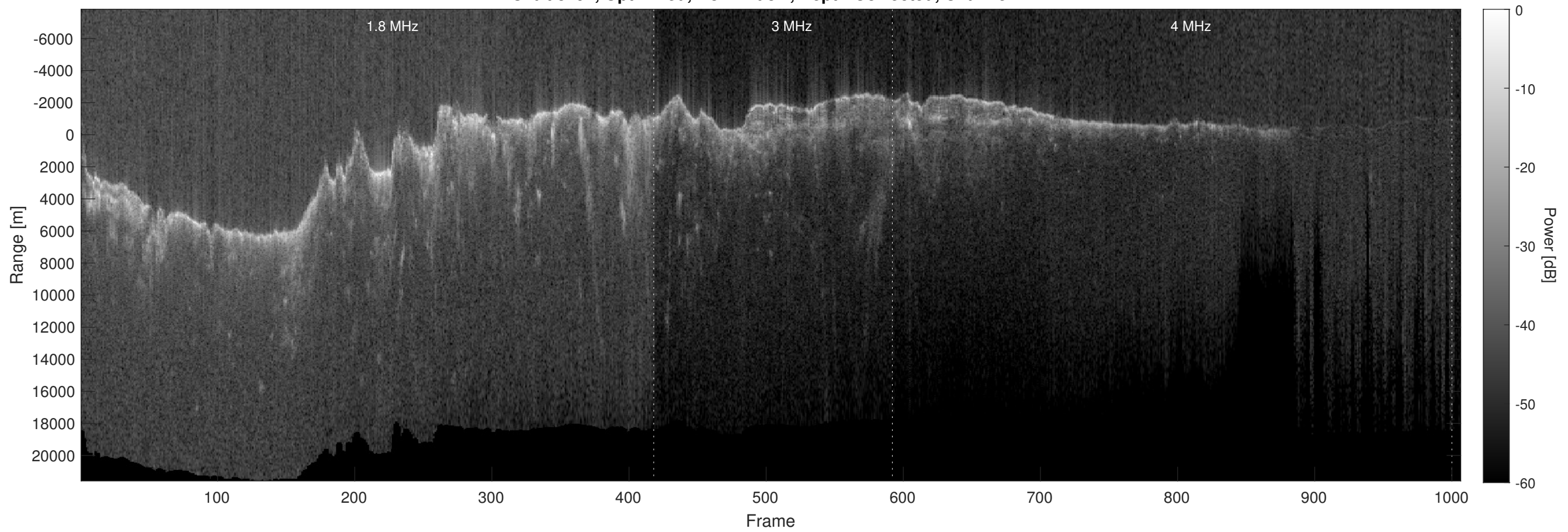
Orbit 8797, Optimized, No Window, Depth-Corrected, Channel 2
