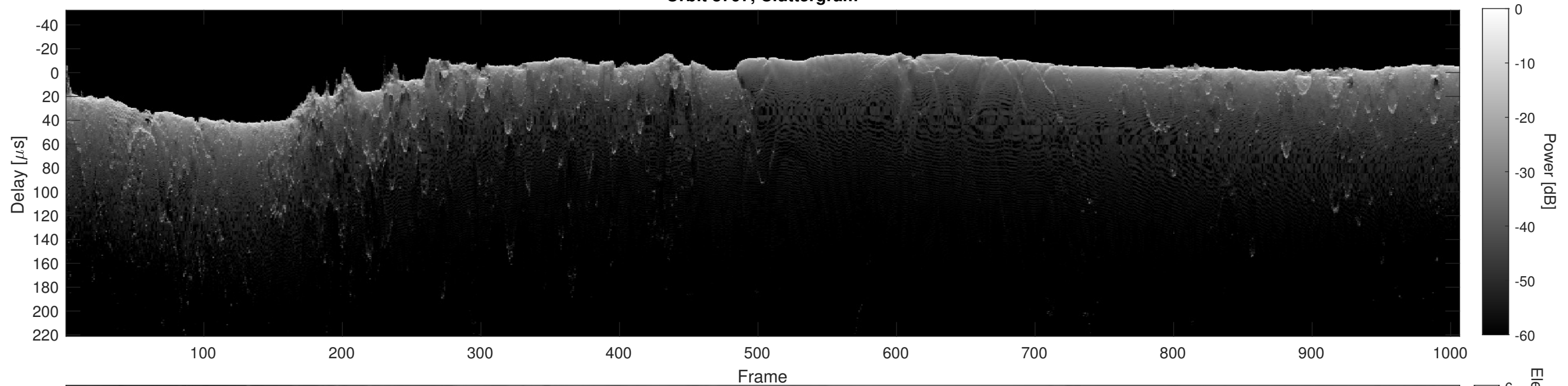
Orbit 8797, Cluttergram
