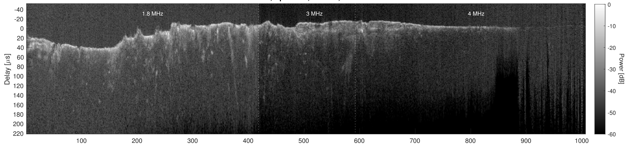
Orbit 8797, Cluttergram
