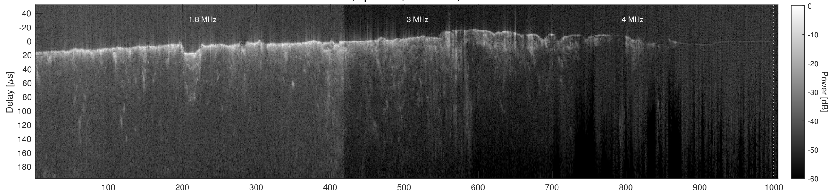
Orbit 8798, Cluttergram
