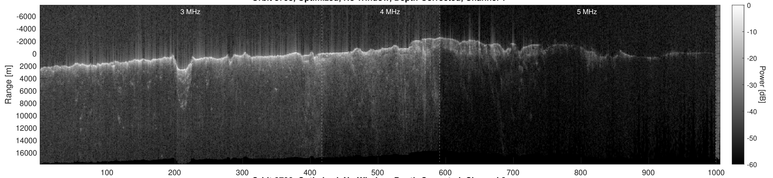
Orbit 8798, Optimized, No Window, Depth-Corrected, Channel 2
