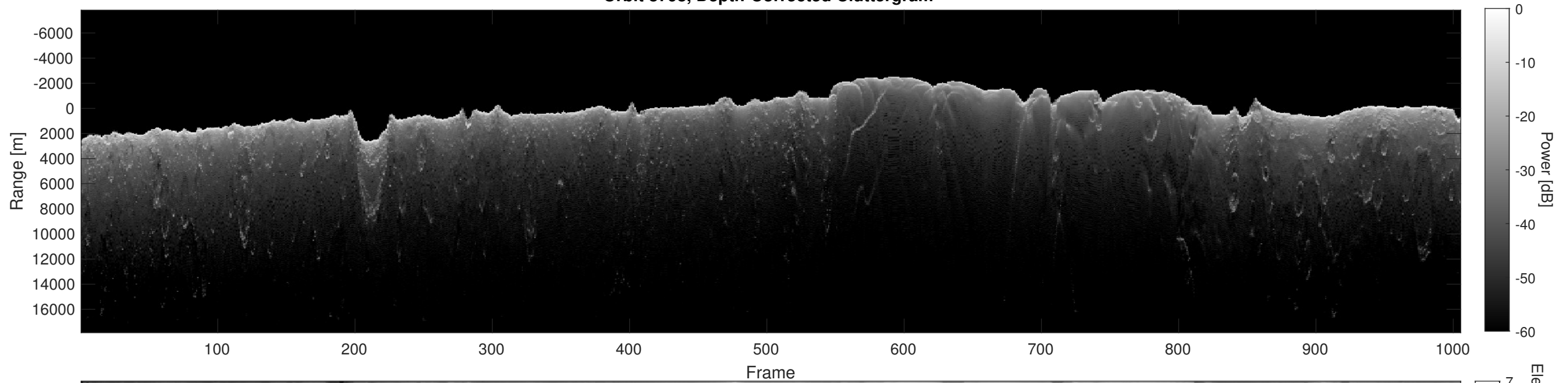
Orbit 8798, Depth-Corrected Cluttergram
