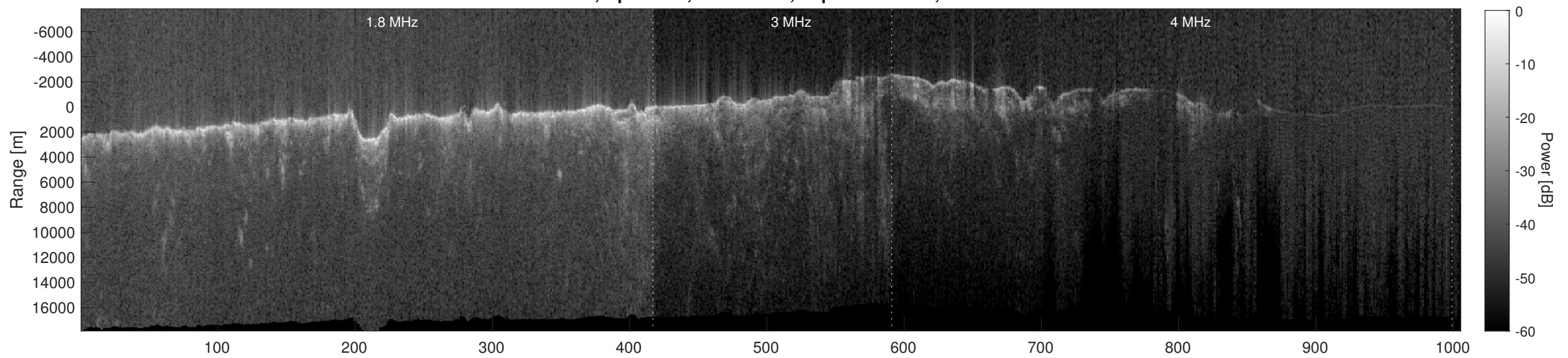
Orbit 8798, Depth-Corrected Cluttergram
