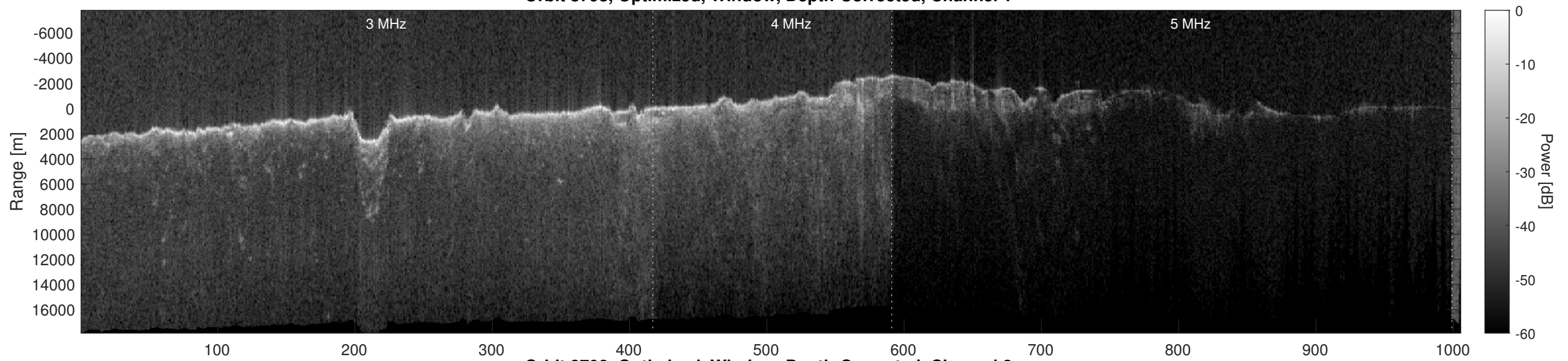
Orbit 8798, Optimized, Window, Depth-Corrected, Channel 2
