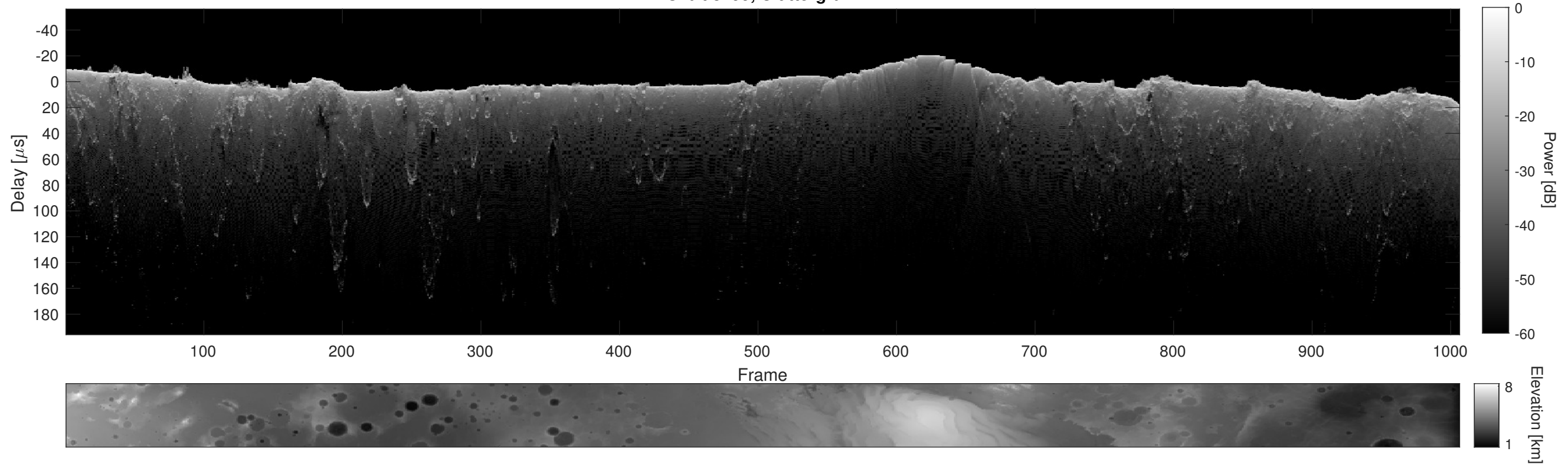
Orbit 8799, Cluttergram
