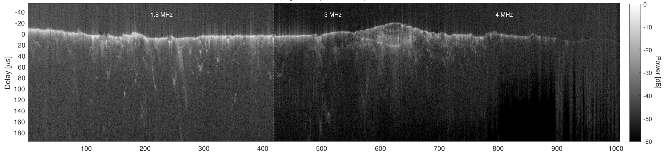
Orbit 8799, Cluttergram
