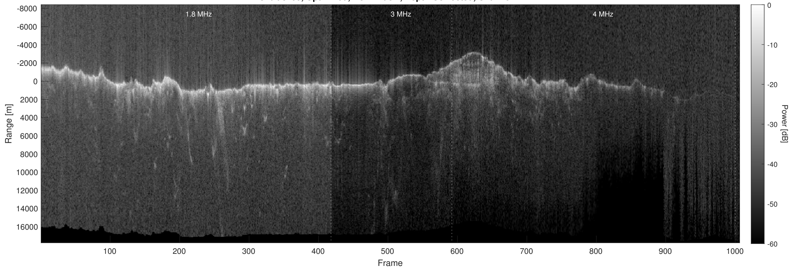
Orbit 8799, Optimized, No Window, Depth-Corrected, Channel 2
