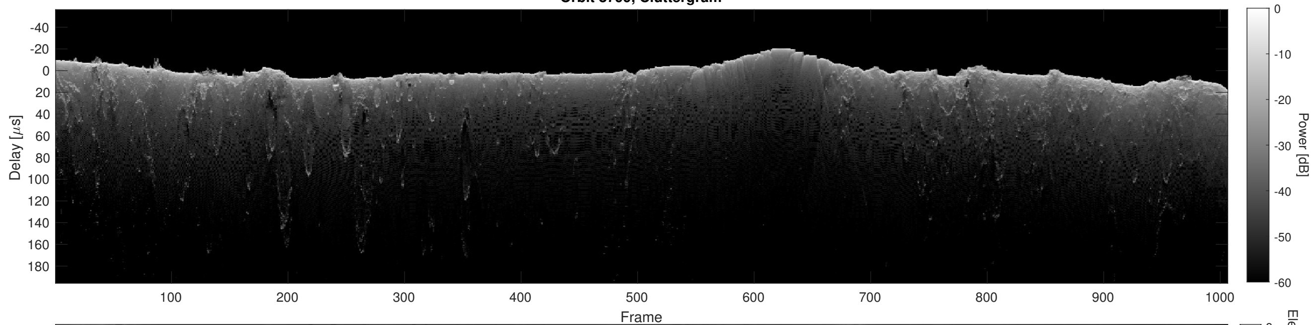
Orbit 8799, Cluttergram
