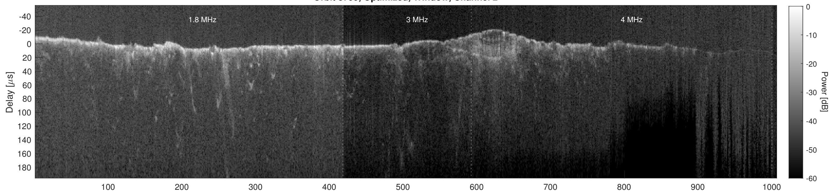
Orbit 8799, Cluttergram
