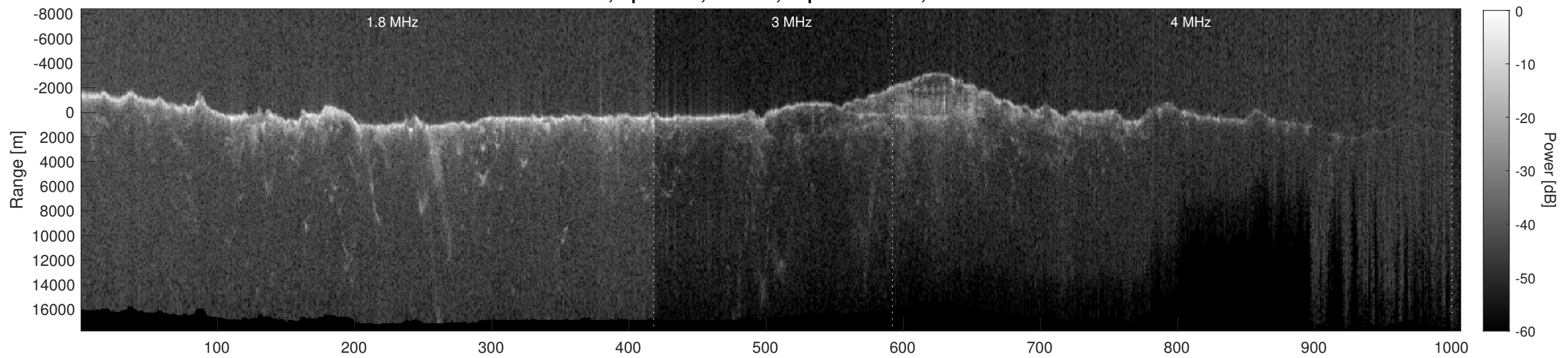
Orbit 8799, Depth-Corrected Cluttergram
