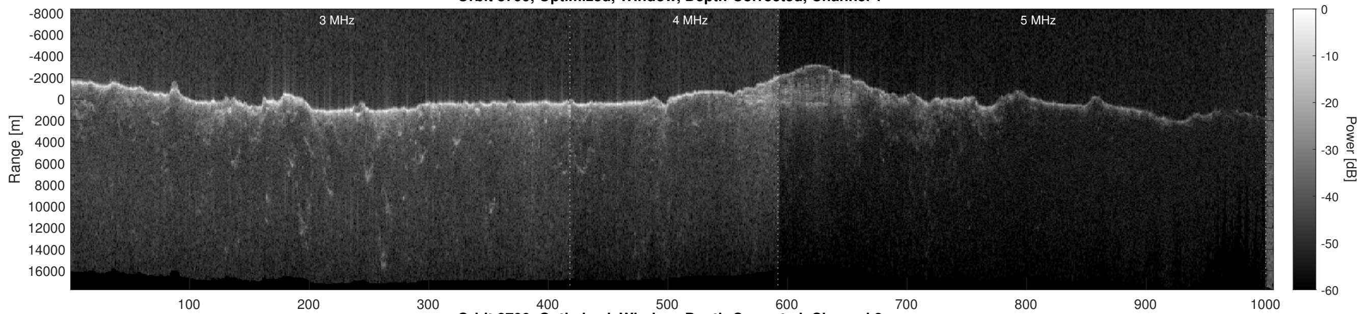
Orbit 8799, Optimized, Window, Depth-Corrected, Channel 2
