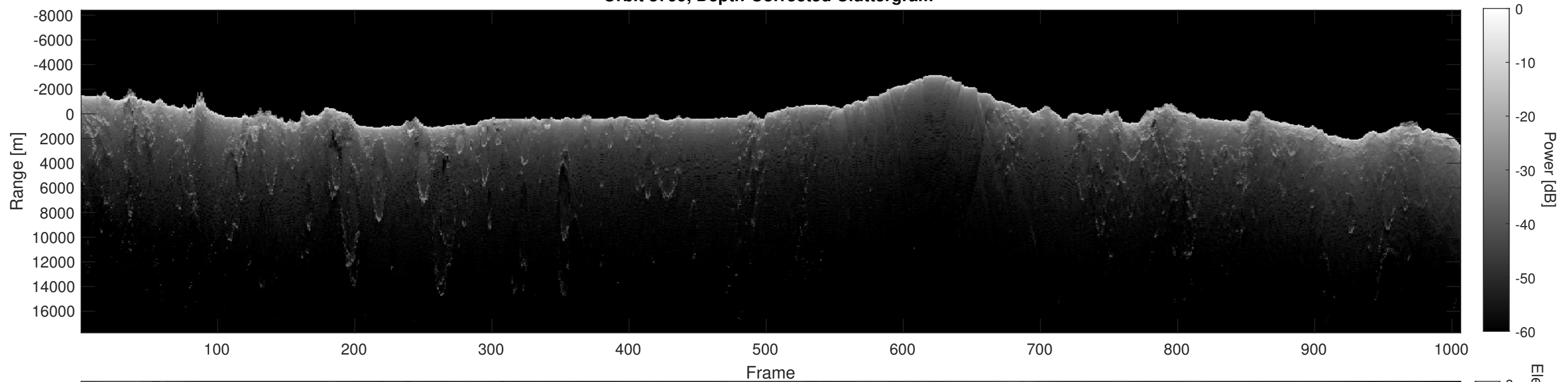
Orbit 8799, Depth-Corrected Cluttergram
