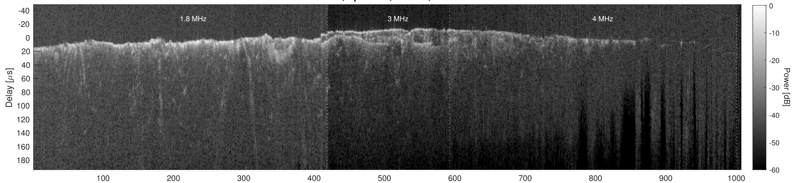
Orbit 8800, Cluttergram
