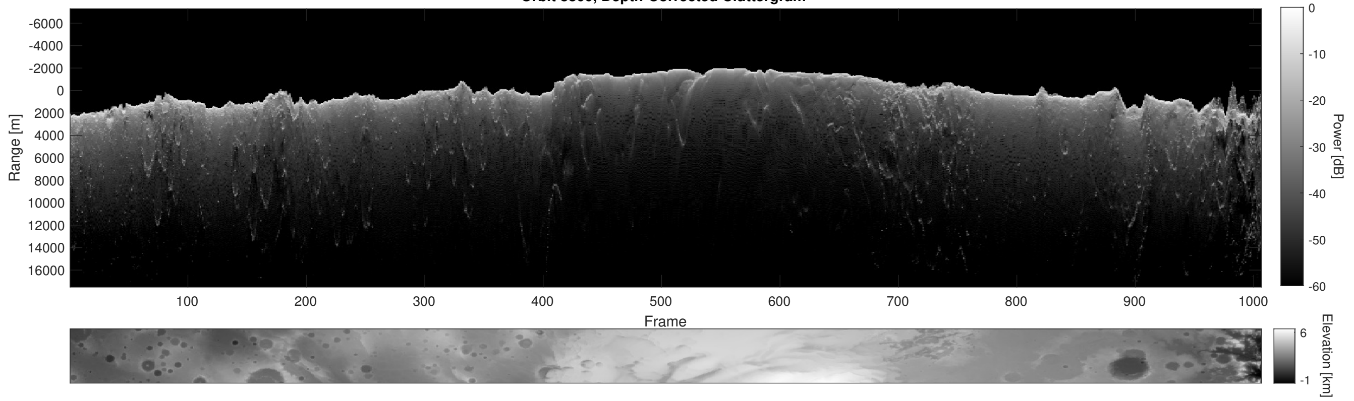
Orbit 8800, Depth-Corrected Cluttergram
