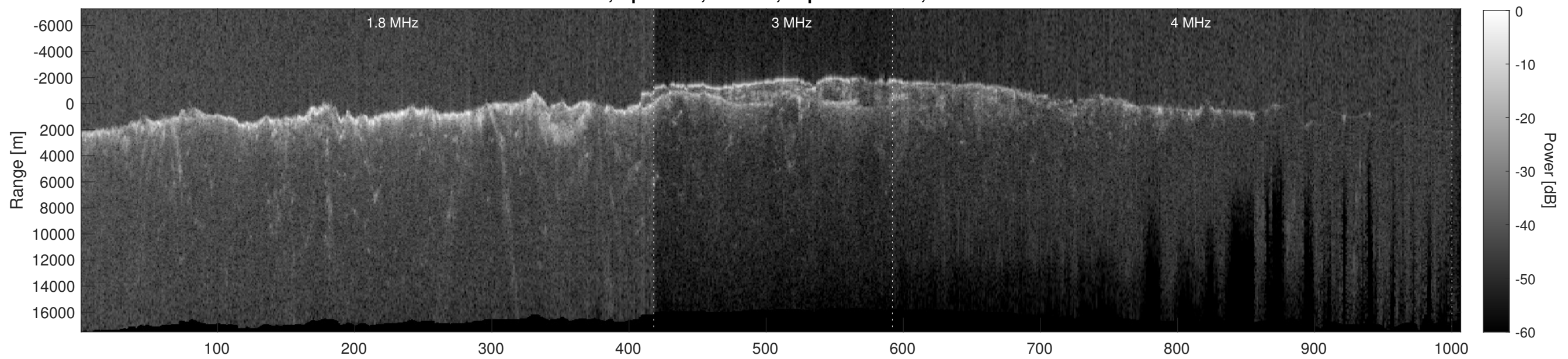
Orbit 8800, Depth-Corrected Cluttergram
