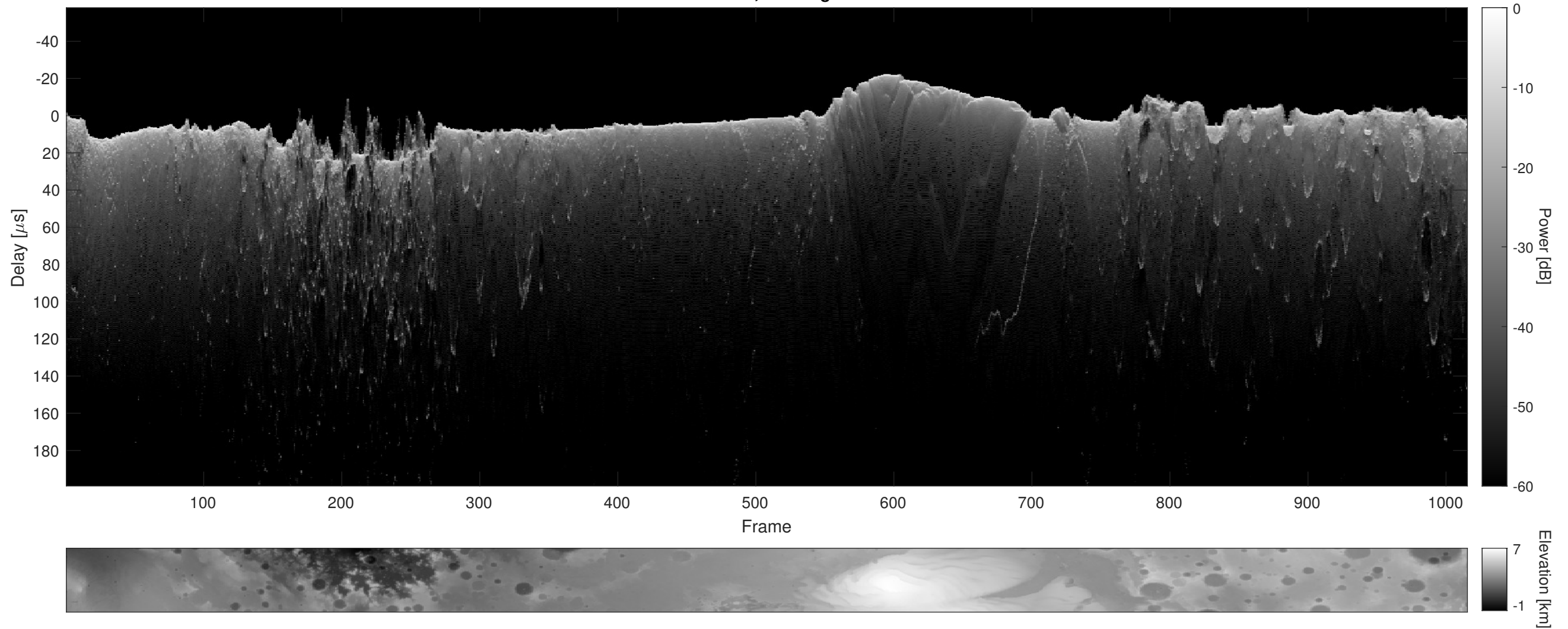
Orbit 8802, Cluttergram
