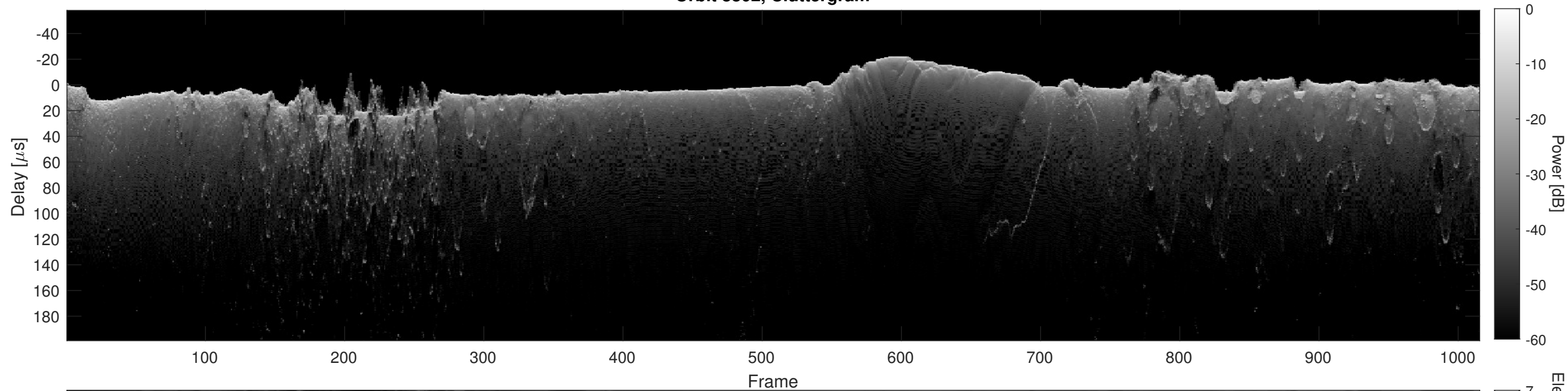
Orbit 8802, Cluttergram
