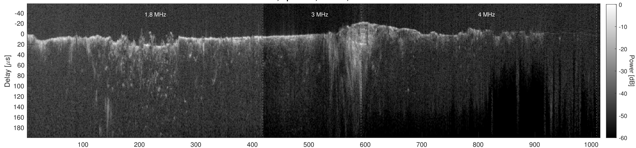
Orbit 8802, Cluttergram
