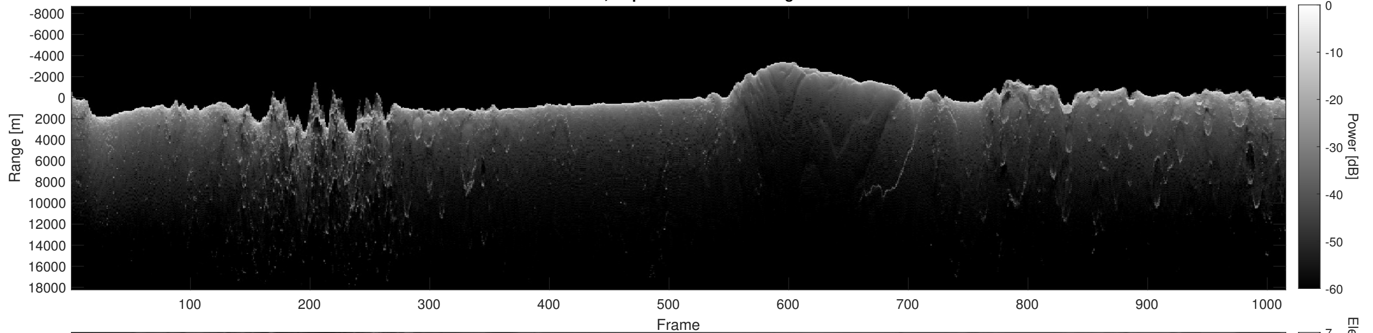
Orbit 8802, Depth-Corrected Cluttergram
