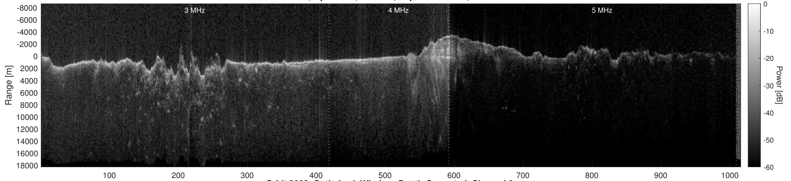
Orbit 8802, Optimized, Window, Depth-Corrected, Channel 2
