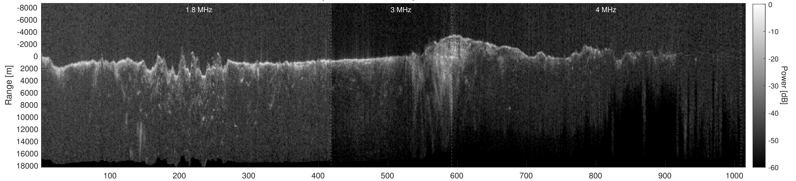
Orbit 8802, Depth-Corrected Cluttergram
