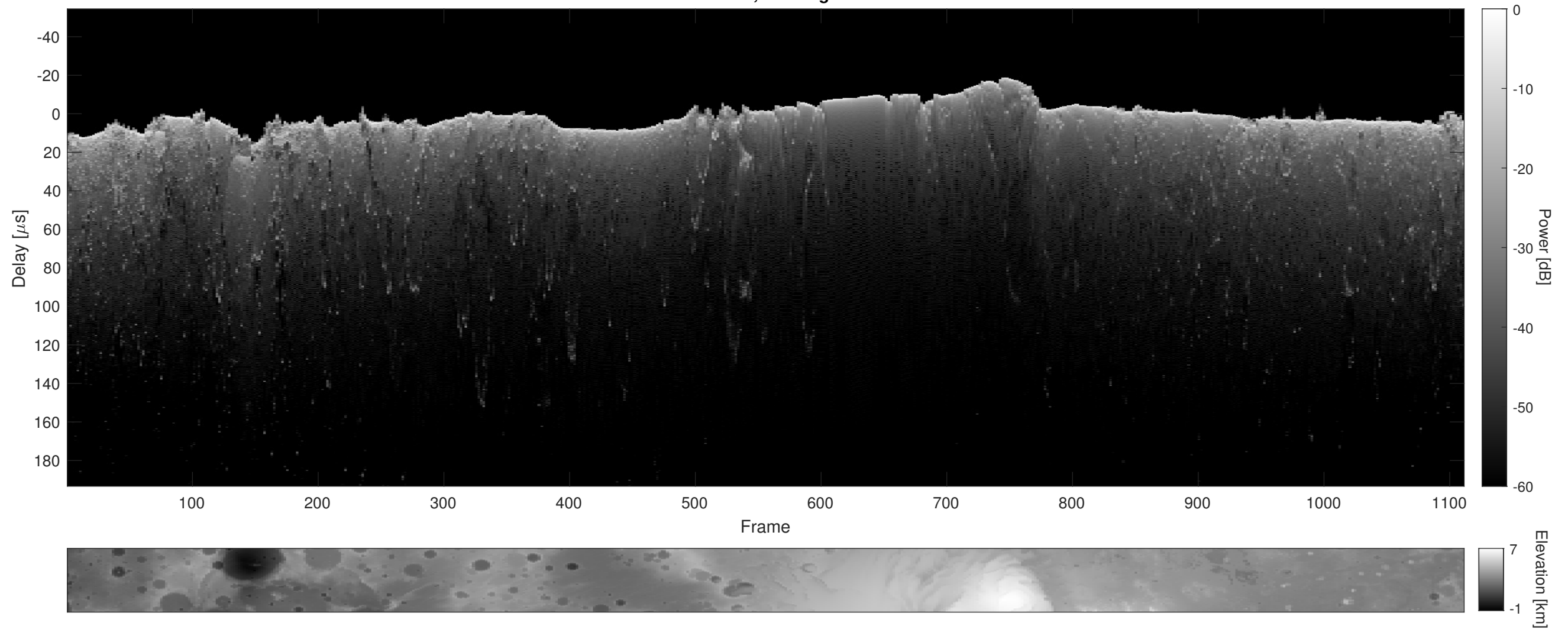
Orbit 8803, Cluttergram
