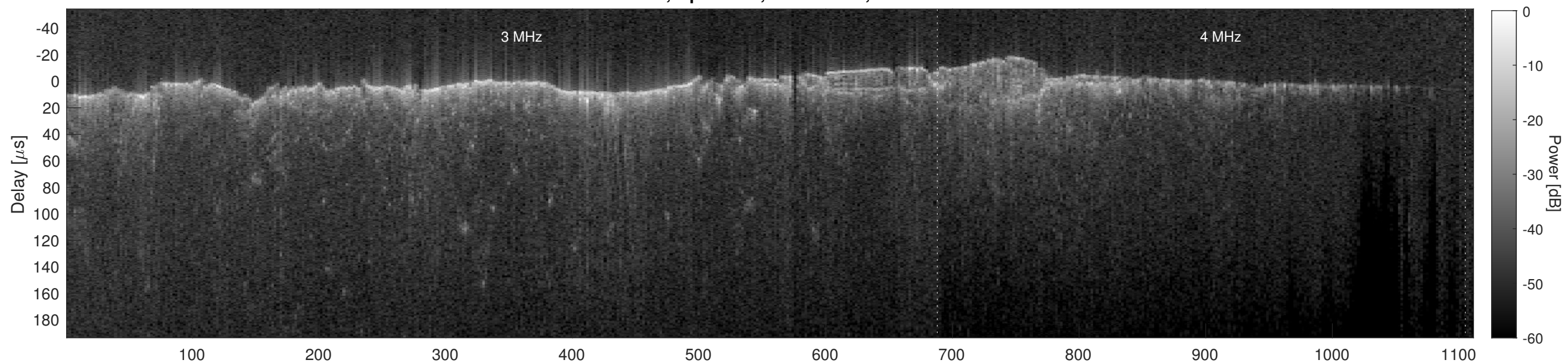
Orbit 8803, Cluttergram
