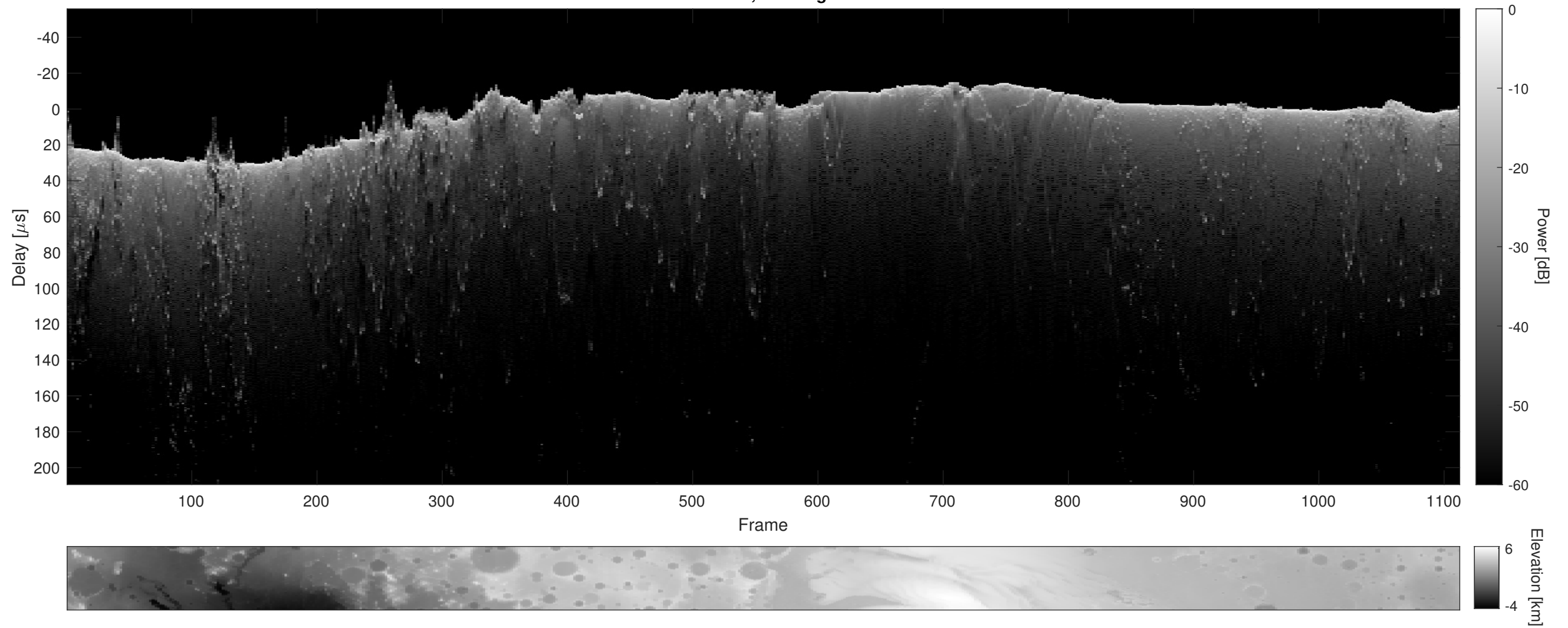
Orbit 8804, Cluttergram
