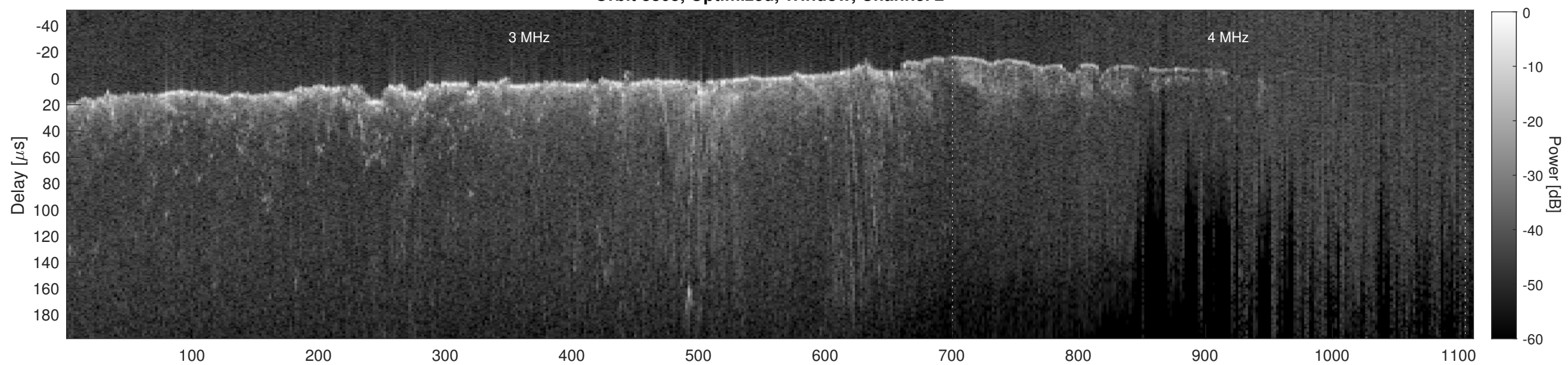
Orbit 8805, Cluttergram
