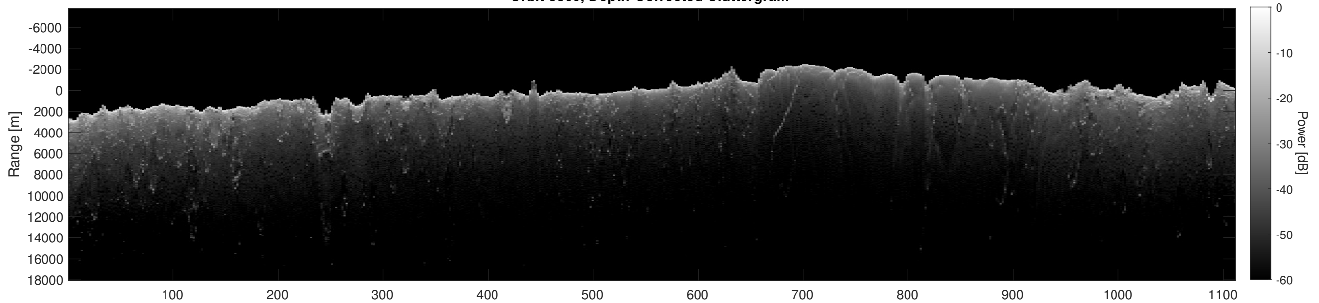
Orbit 8805, Depth-Corrected Cluttergram
