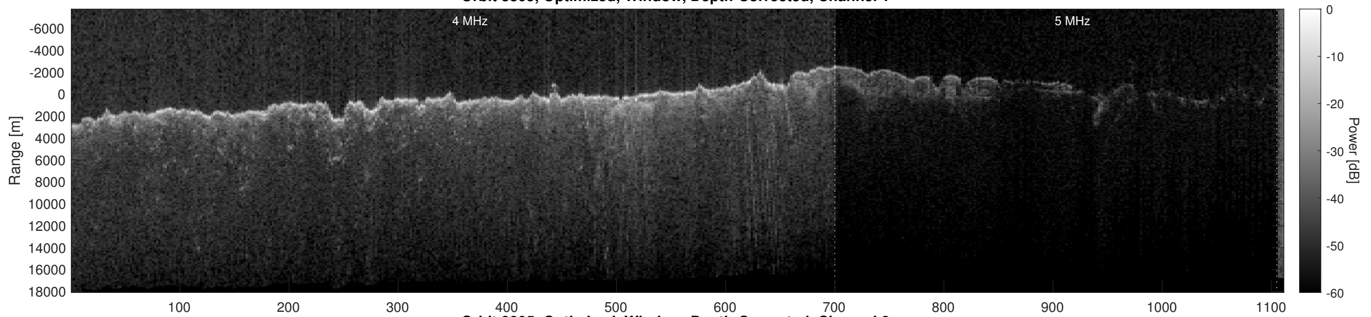
Orbit 8805, Optimized, Window, Depth-Corrected, Channel 2
