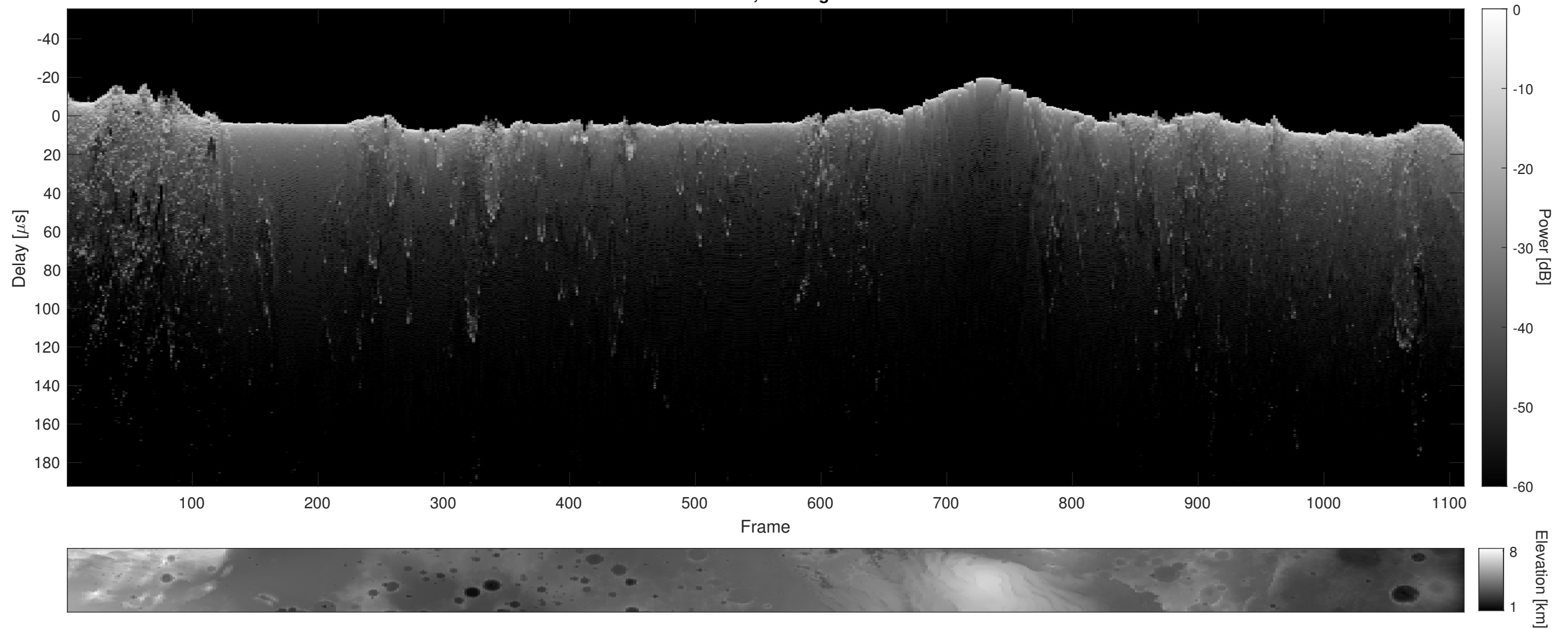
Orbit 8806, Cluttergram
