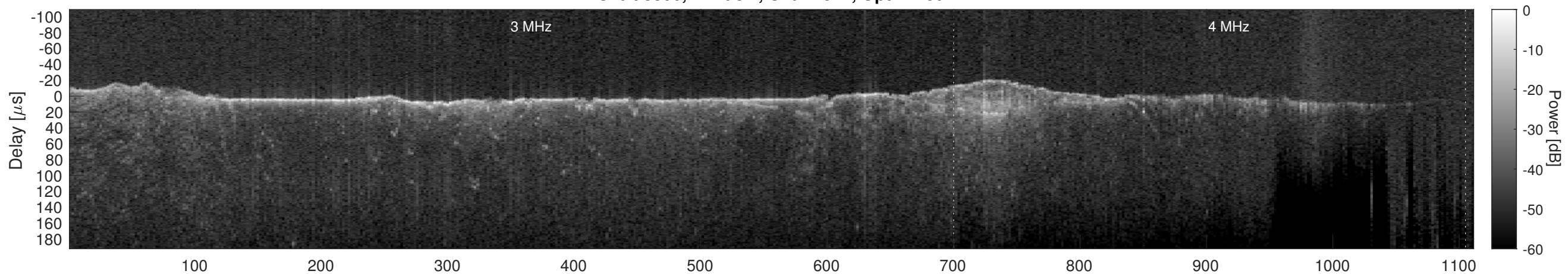
Orbit 8806, Cluttergram
