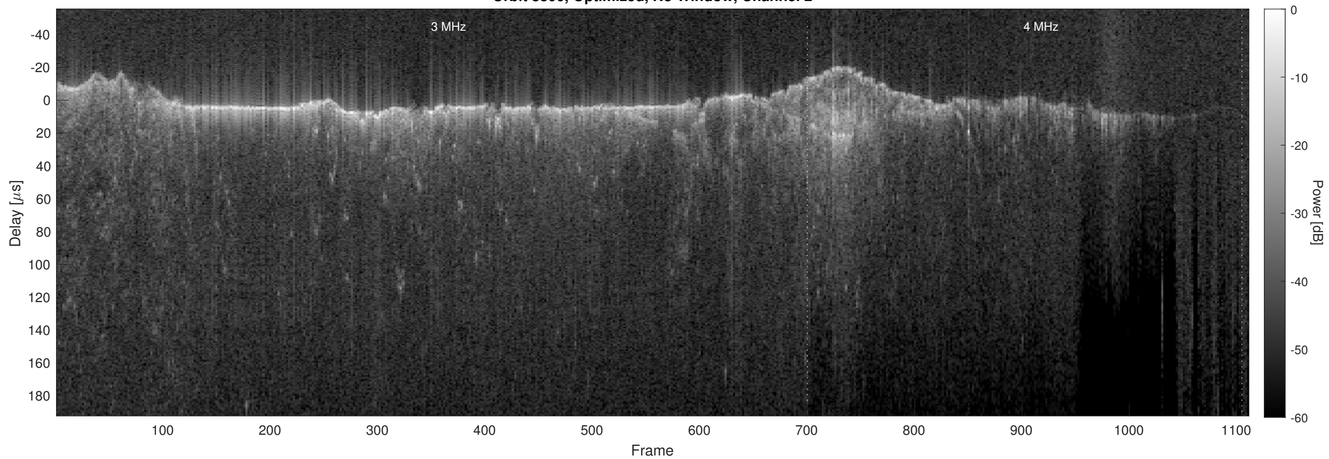
Orbit 8806, Optimized, No Window, Channel 2
