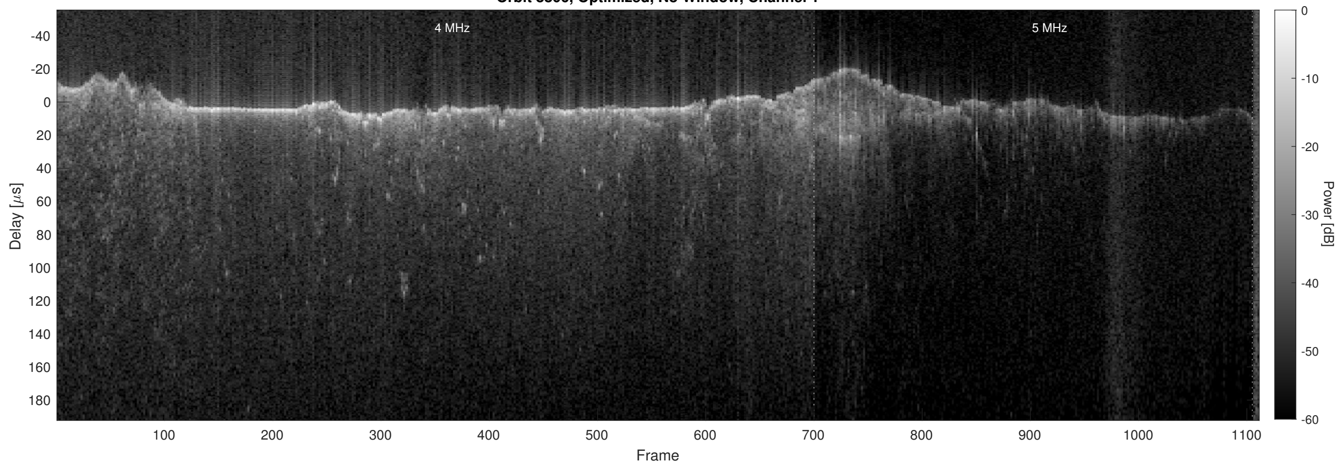
Orbit 8806, Optimized, No Window, Channel 2
