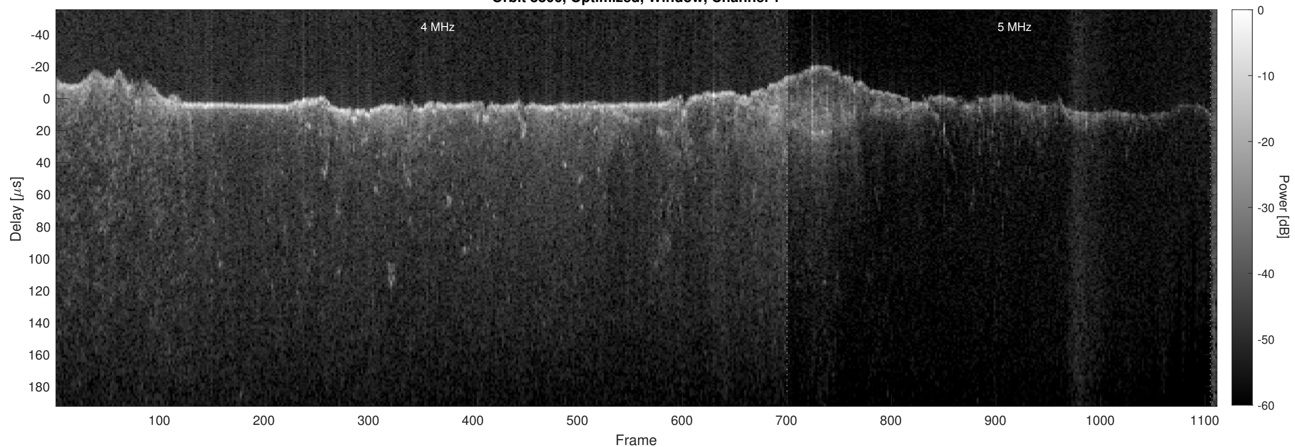
Orbit 8806, Optimized, Window, Channel 2
