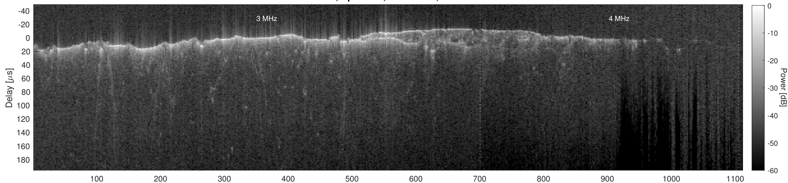
Orbit 8807, Cluttergram
