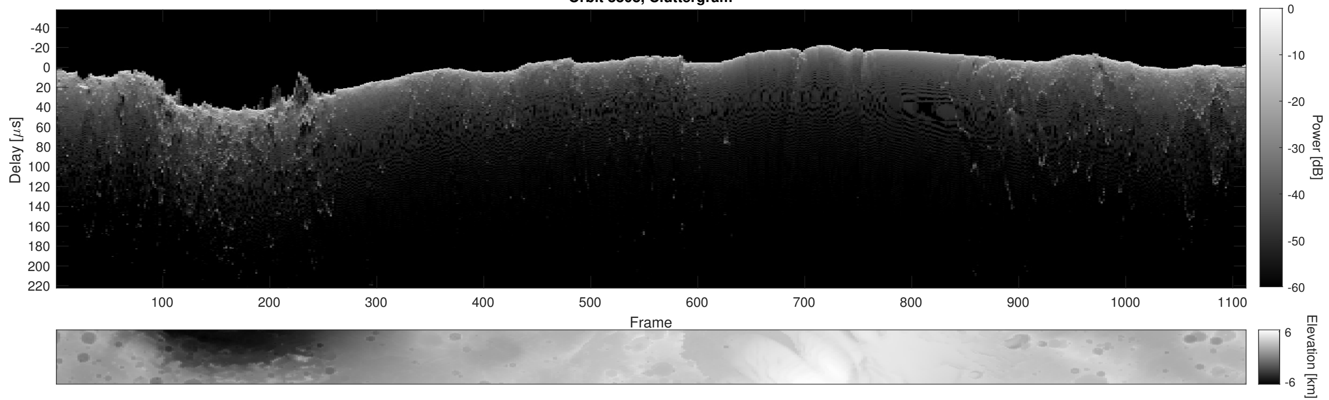
Orbit 8808, Cluttergram
