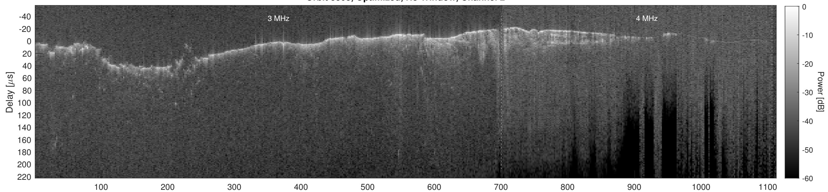
Orbit 8808, Cluttergram
