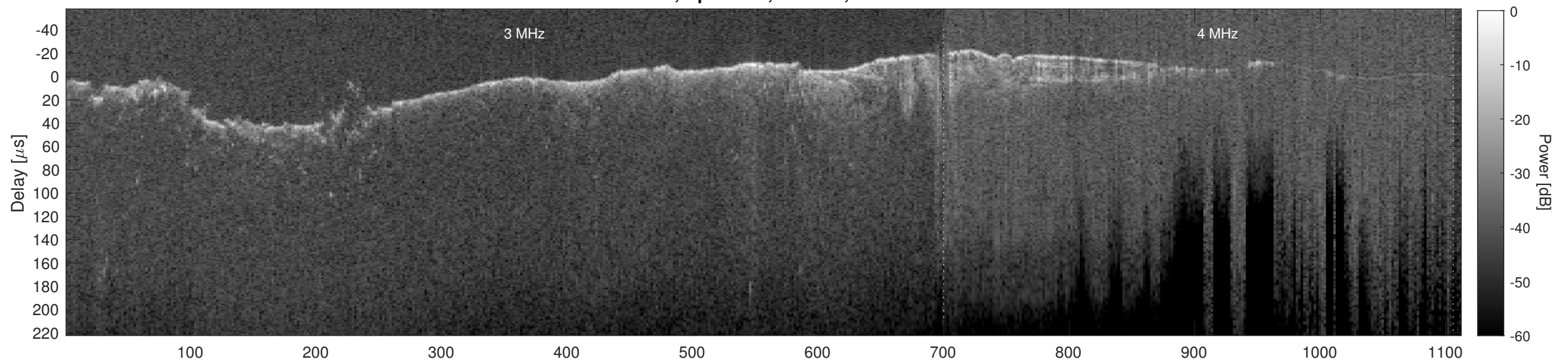
Orbit 8808, Cluttergram
