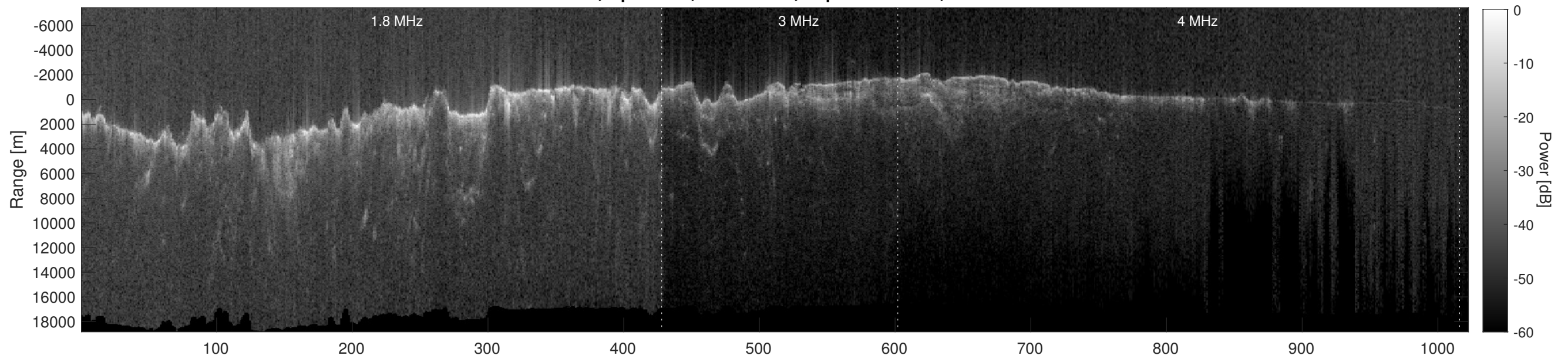
Orbit 8811, Depth-Corrected Cluttergram
