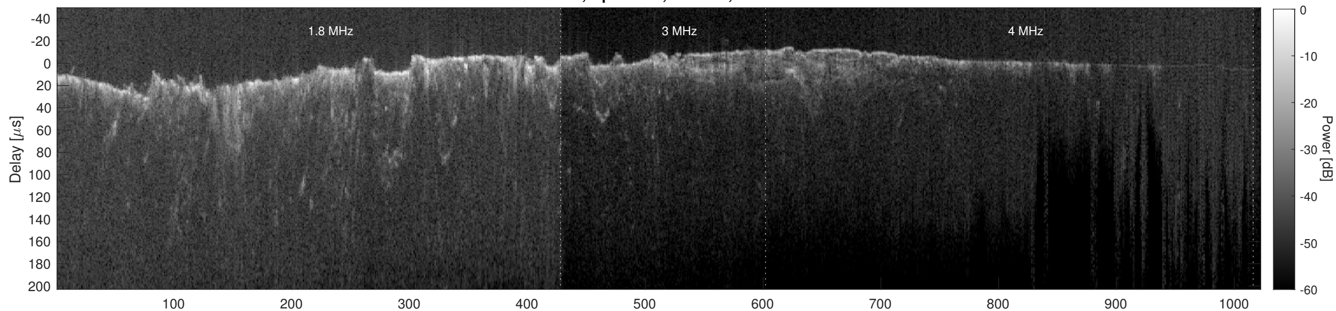
Orbit 8811, Cluttergram
