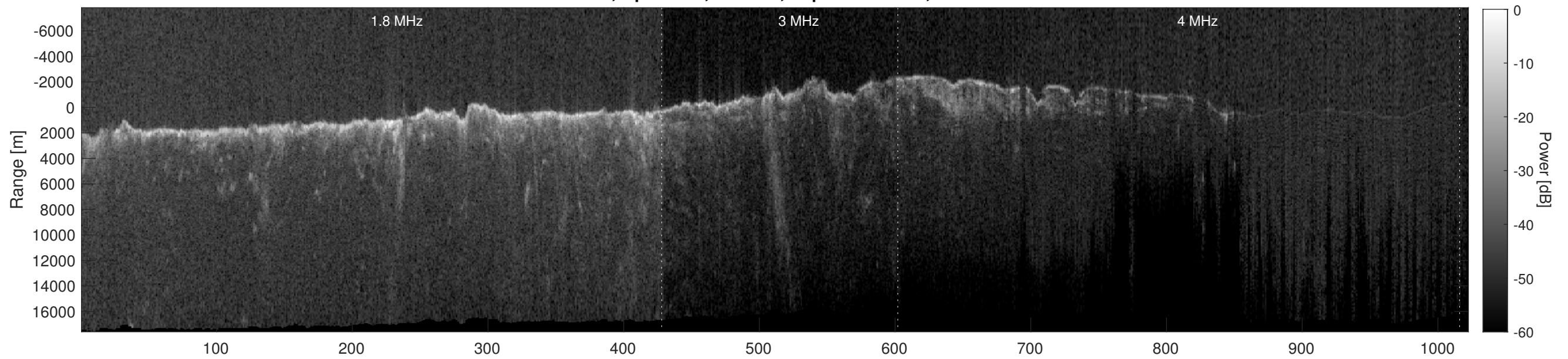
Orbit 8812, Depth-Corrected Cluttergram
